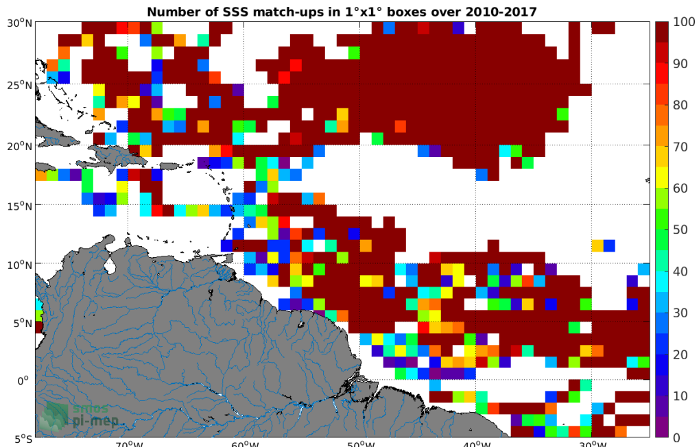
Figure 3: Number of SSS match-ups between Surface drifters SSS and the CCI SSS L4 Merged-OI v2.31 - 7-day running (ESA) SSS product for the Amazon and Orinoco river plumes Pi-MEP region over 1^\circ \times 1^\circ boxes and for the full satellite product period.
