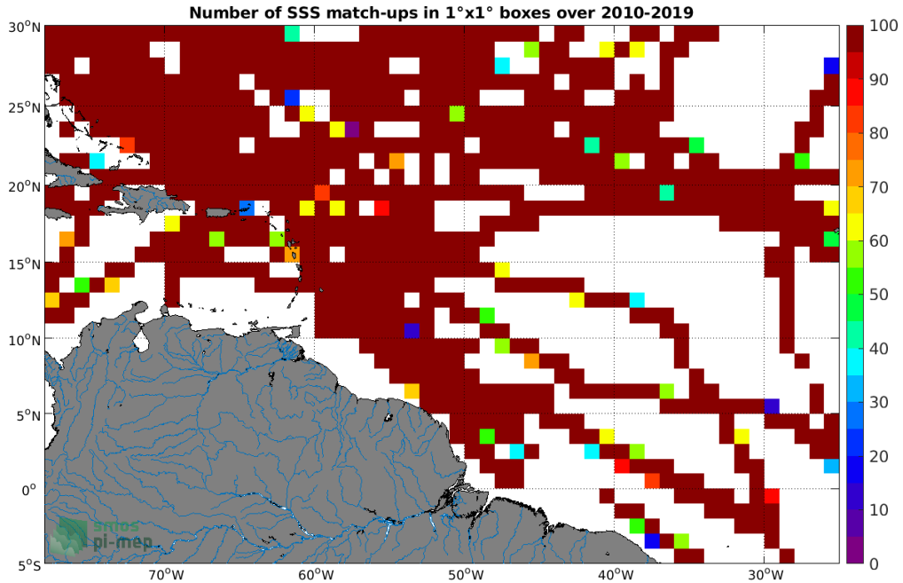
Figure 4: Number of SSS match-ups between TSG (SAMOS) SSS and the CCI SSS L4 Merged-OI v2.31 - 30-day running (ESA) SSS product for the Amazon and Orinoco river plumes Pi-MEP region over 1^\circ \times 1^\circ boxes and for the full satellite product period.
