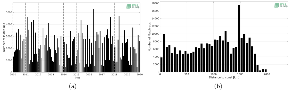
Figure 1: Number of match-ups between TSG (LEGOS-DM) and CCI SSS L4 Merged-OI v2.31 - 30-day running (ESA) SSS as a function of time (a) and as function of the distance to coast (b) over the Amazon and Orinoco river plumes Pi-MEP region and for the full satellite product period.
