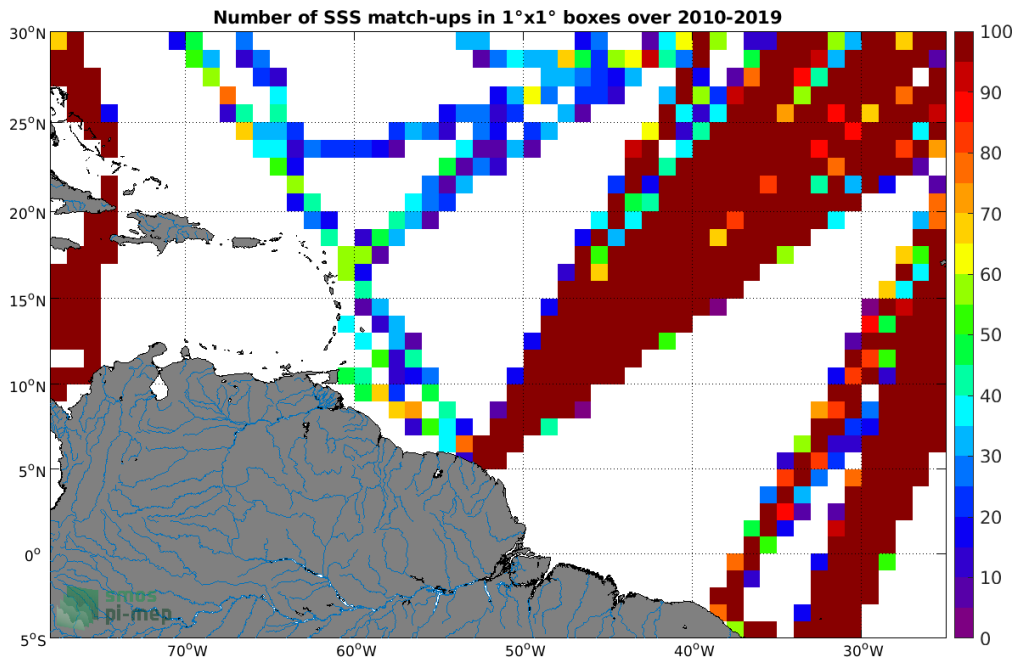
Figure 4: Number of SSS match-ups between TSG (LEGOS-DM) SSS and the CCI SSS L4 Merged-OI v2.31 - 30-day running (ESA) SSS product for the Amazon and Orinoco river plumes Pi-MEP region over 1^\circ \times 1^\circ boxes and for the full satellite product period.
