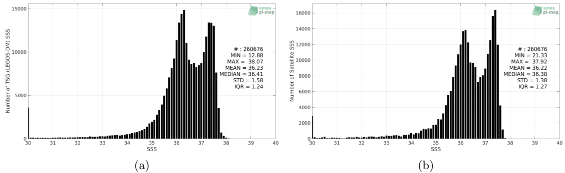
Figure 2: Histograms of SSS from TSG (LEGOS-DM) (a) and CCI SSS L4 Merged-OI v2.31 - 30-day running (ESA) (b) considering all match-up pairs per bins of 0.1 over the Amazon and Orinoco river plumes Pi-MEP region and for the full satellite product period.
