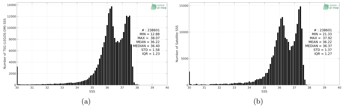
Figure 2: Histograms of SSS from TSG (LEGOS-DM) (a) and CCI L4 Merged-OI v2.31 - 30-day running (ESA) (b) considering all match-up pairs per bins of 0.1 over the Amazon and Orinoco river plumes Pi-MEP region and for the full satellite product period.
