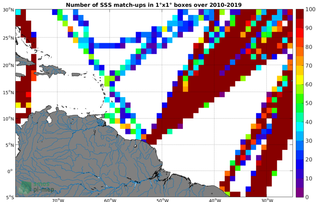
Figure 4: Number of SSS match-ups between TSG (LEGOS-DM) SSS and the CCI L4 Merged-OI v2.31 - 30-day running (ESA) SSS product for the Amazon and Orinoco river plumes Pi-MEP region over 1°x1° boxes and for the full satellite product period.
