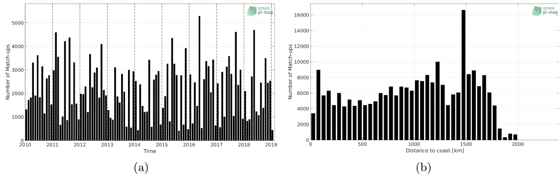
Figure 1: Number of match-ups between TSG (LEGOS-DM) and CCI L4 Merged-OI v2.31 - 30-day running (ESA) SSS as a function of time (a) and as function of the distance to coast (b) over the Amazon and Orinoco river plumes Pi-MEP region and for the full satellite product period.
