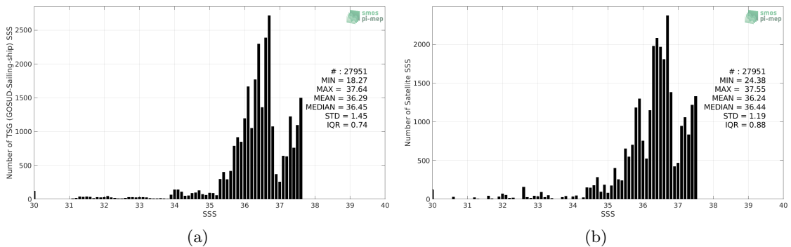
Figure 2: Histograms of SSS from TSG (GOSUD-Sailing-ship) (a) and CCI SSS L4 Merged-OI v2.31 - 30-day running (ESA) (b) considering all match-up pairs per bins of 0.1 over the Amazon and Orinoco river plumes Pi-MEP region and for the full satellite product period.
