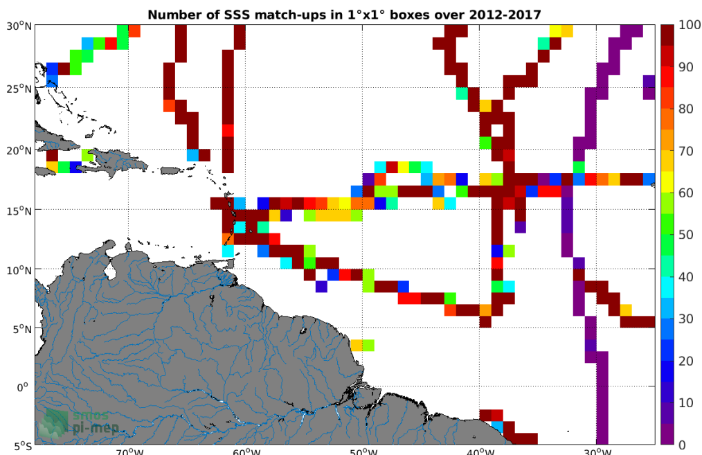
Figure 4: Number of SSS match-ups between TSG (GOSUD-Sailing-ship) SSS and the CCI SSS L4 Merged-OI v2.31 - 30-day running (ESA) SSS product for the Amazon and Orinoco river plumes Pi-MEP region over 1^\circ \times 1^\circ boxes and for the full satellite product period.
