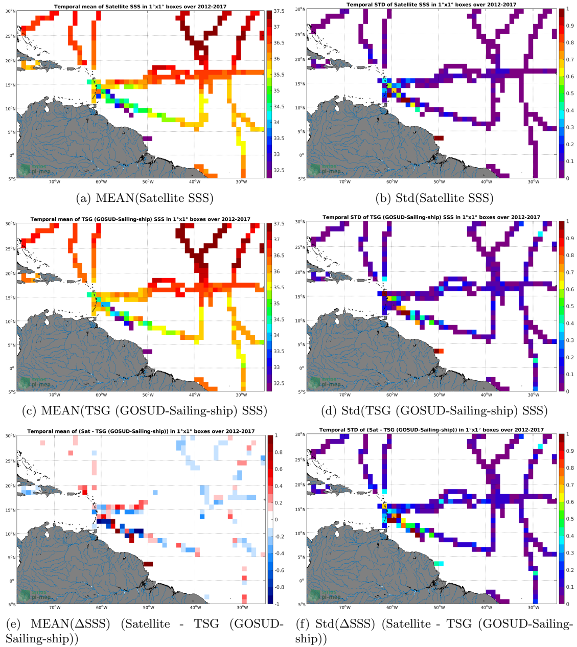
Figure 6: Temporal mean (left) and Std (right) of SSS from CCI SSS L4 Merged-OI v2.31 - 30-day running (ESA) (top), TSG (GOSUD-Sailing-ship) (middle), and of \Delta SSS (Satellite - TSG (GOSUD-Sailing-ship)). Only match-up pairs are used to generate these maps.
