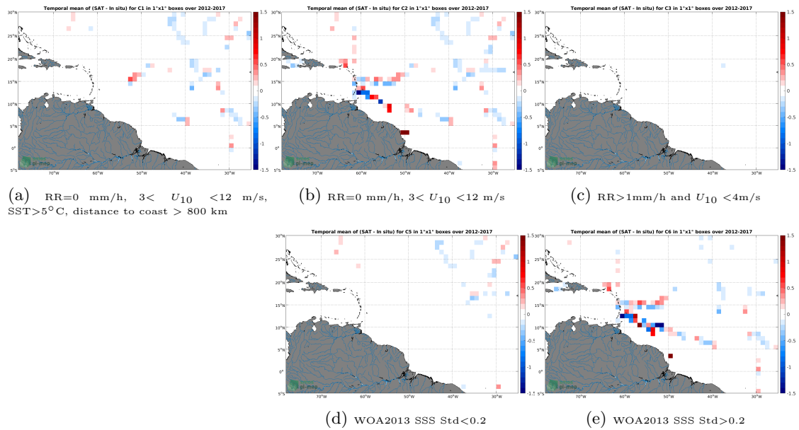
Figure 12: Temporal mean gridded over spatial boxes of size 1^{\circ}\times 1^{\circ} of \Delta SSS (CCI SSS L4 Merged-OI v2.31 - 30-day running (ESA) - TSG (GOSUD-Sailing-ship)) for 5 different subdatasets corresponding to:RR=0 mm/h, 3 < U_{10} < 12 m/s, SST >5^{\circ}\text{C} , distance to coast > 800 km (a), RR=0 mm/h, 3 < U_{10} < 12 m/s (b), RR >1 mm/h and U_{10} < 4 m/s (c), WOA2013 SSS Std <0.2 (d), WOA2013 SSS Std >0.2 (e).
