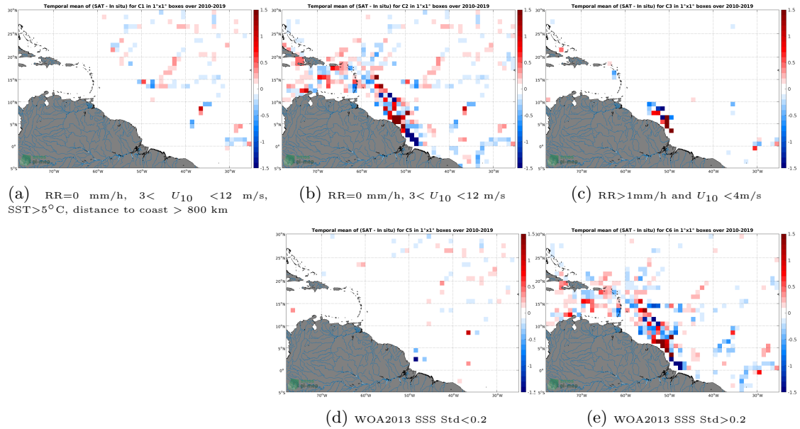
Figure 12: Temporal mean gridded over spatial boxes of size 1^{\circ}\times 1^{\circ} of \Delta SSS (CCI SSS L4 Merged-OI v2.31 - 30-day running (ESA) - TSG (GOSUD-Research-vessel)) for 5 different subdatasets corresponding to:RR=0 mm/h, 3 < U_{10} < 12 m/s, SST >5^{\circ}\text{C} , distance to coast > 800 km (a), RR=0 mm/h, 3 < U_{10} < 12 m/s (b), RR >1 mm/h and U_{10} < 4 m/s (c), WOA2013 SSS Std <0.2 (d), WOA2013 SSS Std >0.2 (e).
