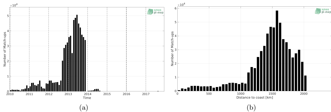
Figure 1: Number of match-ups between Surface drifters and CCI SSS L4 Merged-OI v2.31 - 30-day running (ESA) SSS as a function of time (a) and as function of the distance to coast (b) over the Amazon and Orinoco river plumes Pi-MEP region and for the full satellite product period.
