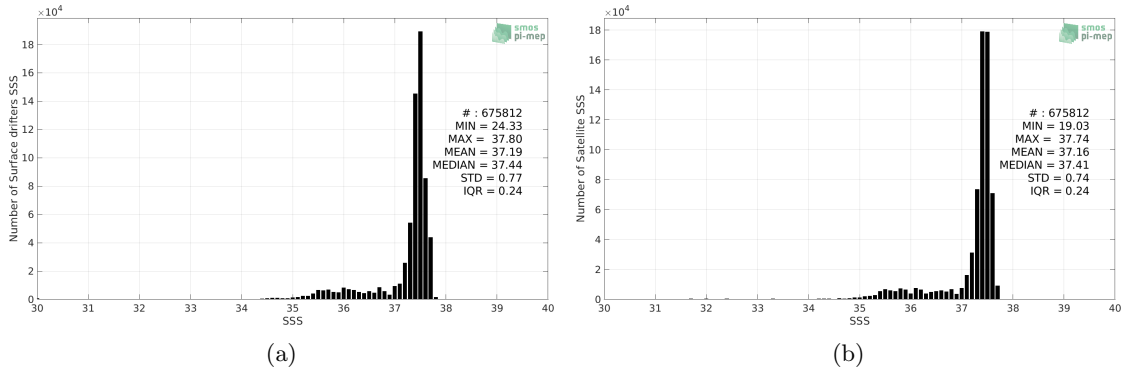
Figure 2: Histograms of SSS from Surface drifters (a) and CCI SSS L4 Merged-OI v2.31 - 30-day running (ESA) (b) considering all match-up pairs per bins of 0.1 over the Amazon and Orinoco river plumes Pi-MEP region and for the full satellite product period.
