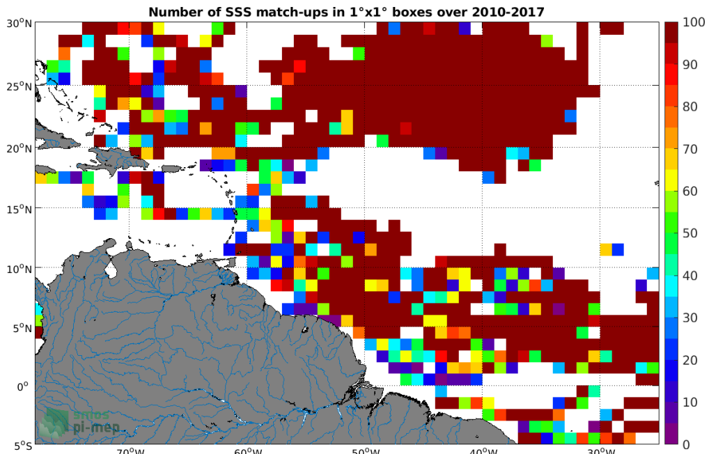
Figure 3: Number of SSS match-ups between Surface drifters SSS and the CCI SSS L4 Merged-OI v2.31 - 30-day running (ESA) SSS product for the Amazon and Orinoco river plumes Pi-MEP region over 1^\circ \times 1^\circ boxes and for the full satellite product period.
