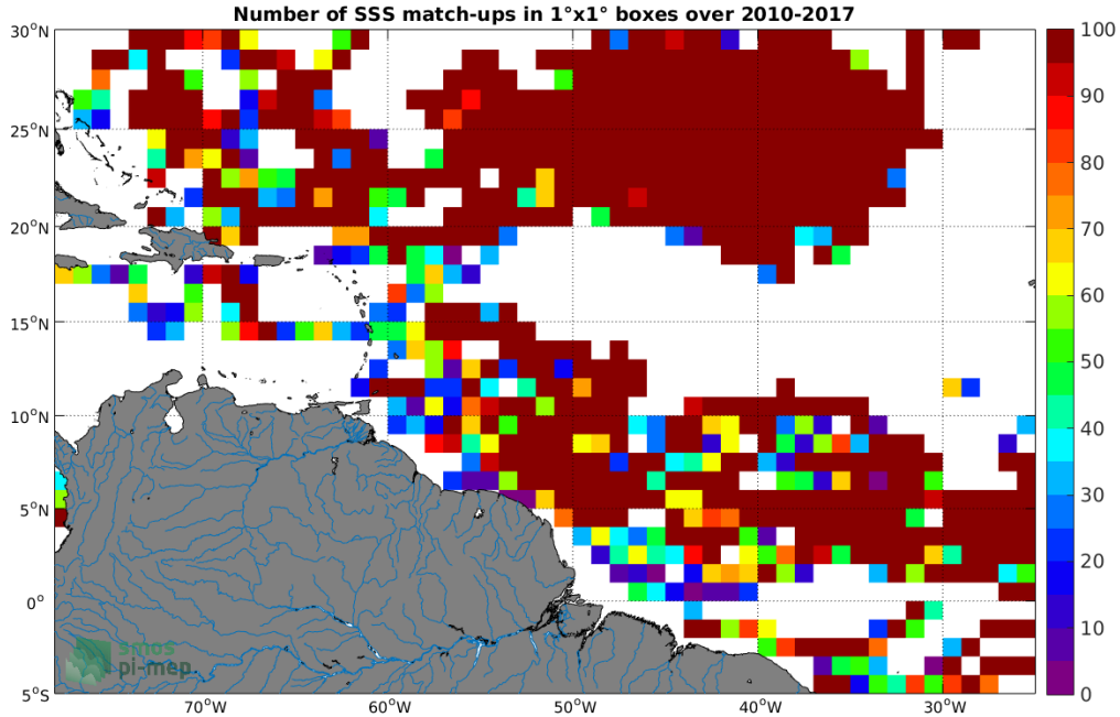
Figure 3: Number of SSS match-ups between Surface drifters SSS and the CCI L4 Merged-OI v2.31 - 30-day running (ESA) SSS product for the Amazon and Orinoco river plumes Pi-MEP region over 1°x1° boxes and for the full satellite product period.
