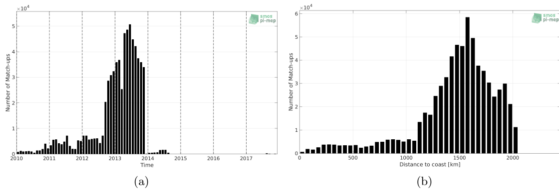
Figure 1: Number of match-ups between Surface drifters and CCI L4 Merged-OI v2.31 - 30-day running (ESA) SSS as a function of time (a) and as function of the distance to coast (b) over the Amazon and Orinoco river plumes Pi-MEP region and for the full satellite product period.
