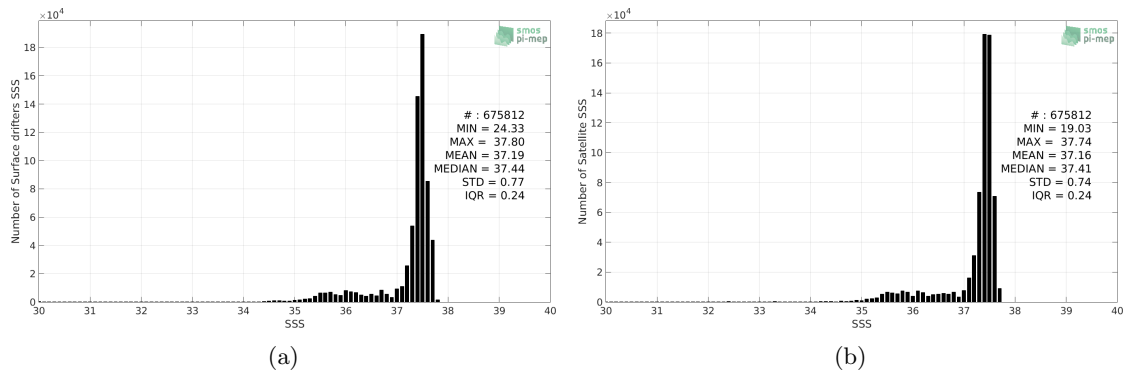
Figure 2: Histograms of SSS from Surface drifters (a) and CCI L4 Merged-OI v2.31 - 30-day running (ESA) (b) considering all match-up pairs per bins of 0.1 over the Amazon and Orinoco river plumes Pi-MEP region and for the full satellite product period.
