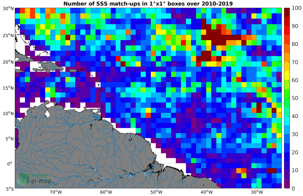
Figure 4: Number of SSS match-ups between Argo SSS and the CCI SSS L4 Merged-OI v2.31 - 30-day running (ESA) SSS product for the Amazon and Orinoco river plumes Pi-MEP region over 1^\circ \times 1^\circ boxes and for the full satellite product period.
