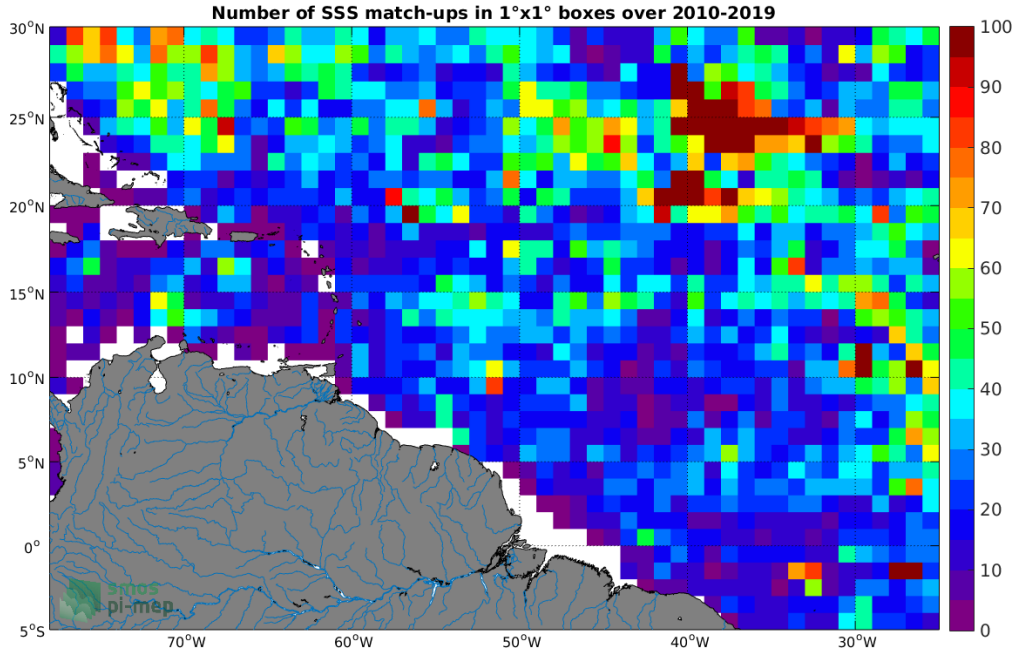
Figure 4: Number of SSS match-ups between Argos SSS and the CCI SSS L4 Merged-OI v2.31 - 30-day running (ESA) SSS product for the Amazon and Orinoco river plumes Pi-MEP region over 1°x1° boxes and for the full satellite product period.
