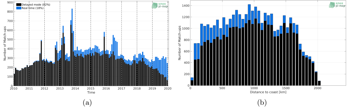
Figure 1: Number of match-ups between Argo and CCI SSS L4 Merged-OI v2.31 - 30-day running (ESA) SSS as a function of time (a) and as function of the distance to coast (b) over the Amazon and Orinoco river plumes Pi-MEP region and for the full satellite product period.
