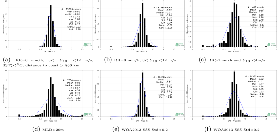
Figure 13: Normalized histogram of \Delta\text{SSS} (CCI SSS L4 Merged-OI v2.31 - 30-day running (ESA) - Argo) for 6 different subdatasets corresponding to: RR=0 mm/h, 3 < U_{10} < 12 m/s, SST>5°C, distance to coast > 800 km (a), RR=0 mm/h, 3 < U_{10} < 12 m/s (b), RR>1mm/h and U_{10} < 4 m/s (c), MLD<20m (d), WOA2013 SSS Std<0.2 (e), WOA2013 SSS Std>0.2 (f).
