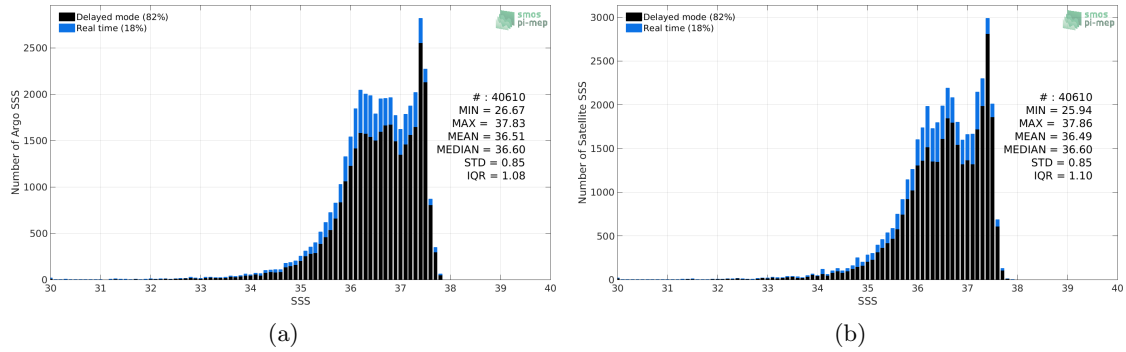
Figure 2: Histograms of SSS from Argo (a) and CCI SSS L4 Merged-OI v2.31 - 30-day running (ESA) (b) considering all match-up pairs per bins of 0.1 over the Amazon and Orinoco river plumes Pi-MEP region and for the full satellite product period.
