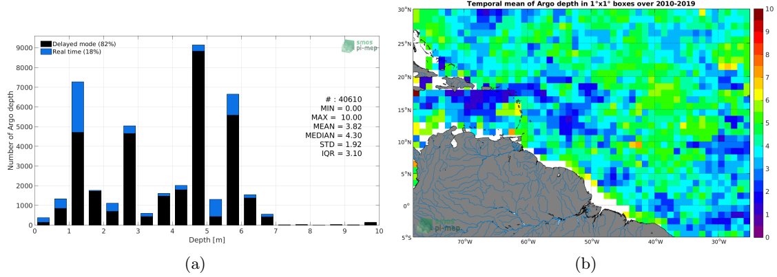
Figure 3: Histograms of the depth of the upper level SSS measurements from Argos in the Match-up DataBase for the Amazon and Orinoco river plumes Pi-MEP region (a) and temporal mean spatial distribution of pressure of the in situ SSS data over 1°x1° boxes and for the full satellite product period (b).
