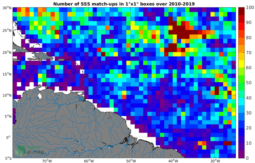
Figure 4: Number of SSS match-ups between Argo SSS and the CCI L4 Merged-OI v2.31 - 30-day running (ESA) SSS product for the Amazon and Orinoco river plumes Pi-MEP region over 1°x1° boxes and for the full satellite product period.
