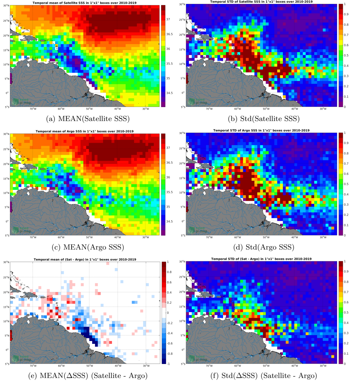
Figure 6: Temporal mean (left) and Std (right) of SSS from CCI L4 Merged-OI v2.31 - 30-day running (ESA) (top), Argo (middle), and of ΔSSS (Satellite - Argo). Only match-up pairs are used to generate these maps.
