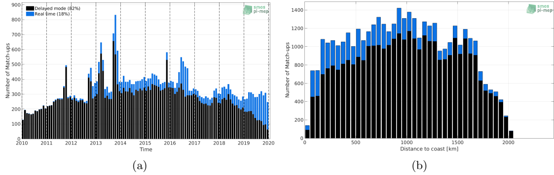
Figure 1: Number of match-ups between Argo and CCI L4 Merged-OI v2.31 - 30-day running (ESA) SSS as a function of time (a) and as function of the distance to coast (b) over the Amazon and Orinoco river plumes Pi-MEP region and for the full satellite product period.
