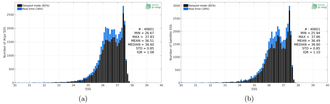
Figure 2: Histograms of SSS from Argo (a) and CCI L4 Merged-OI v2.31 - 30-day running (ESA) (b) considering all match-up pairs per bins of 0.1 over the Amazon and Orinoco river plumes Pi-MEP region and for the full satellite product period.
