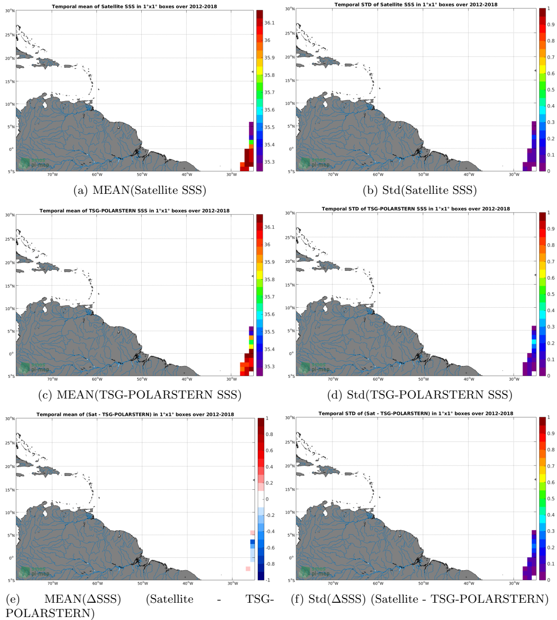
Figure 6: Temporal mean (left) and Std (right) of SSS from CCI-L4-ESA-MERGED-OI-V1.8-30DAY-RUNNING (top), TSG-POLARSTERN (middle), and of \Delta SSS (Satellite - TSG-POLARSTERN). Only match-up pairs are used to generate these maps.
