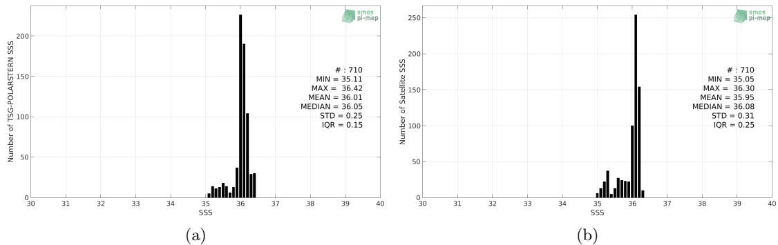
Figure 2: Histograms of SSS from TSG-POLARSTERN (a) and CCI-L4-ESA-MERGED-OI-V1.8-30DAY-RUNNING (b) considering all match-up pairs per bins of 0.1 over the Amazon and Orinoco river plumes Pi-MEP region and for the full satellite product period.
