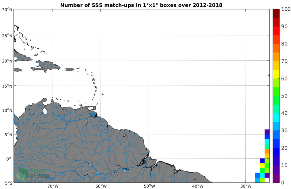
Figure 4: Number of SSS match-ups between TSG-POLARSTERN SSS and the CCI-L4-ESA-MERGED-OI-V1.8-30DAY-RUNNING SSS product for the Amazon and Orinoco river plumes Pi-MEP region over 1^\circ \times 1^\circ boxes and for the full satellite product period.
