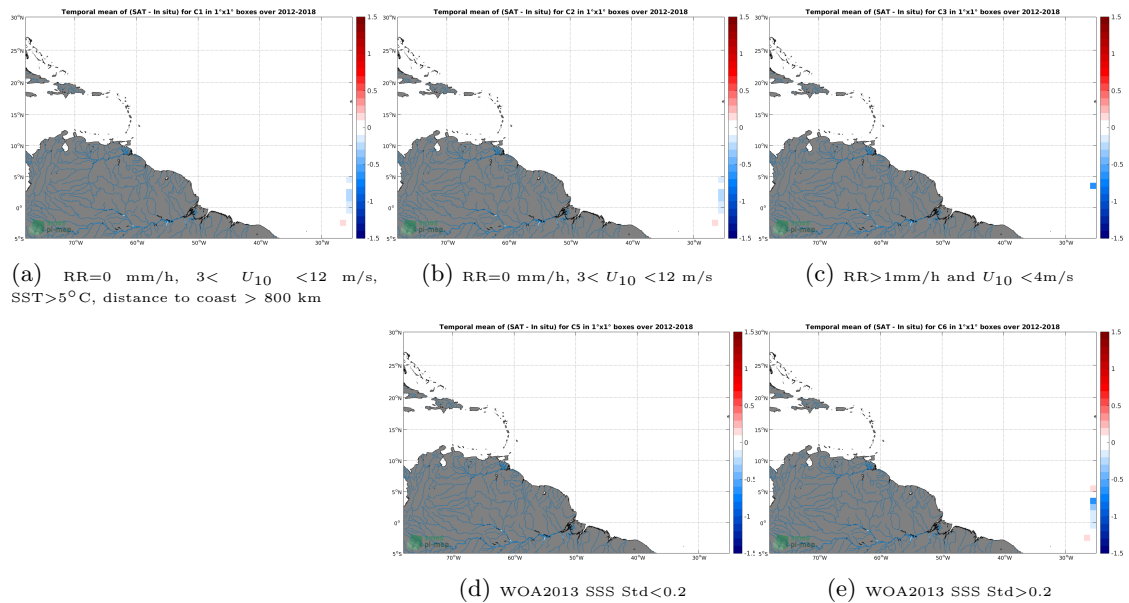
Figure 12: Temporal mean gridded over spatial boxes of size 1^\circ \times 1^\circ of \Delta SSS (CCI-L4-ESAMERGED-OI-V1.8-30DAY-RUNNING - TSG-POLARSTERN) for 5 different subdatasets corresponding to:RR=0 mm/h, 3 < U_{10} < 12 m/s, SST >5^\circ\text{C} , distance to coast > 800 km (a), RR=0 mm/h, 3 < U_{10} < 12 m/s (b), RR >1 mm/h and U_{10} < 4 m/s (c), WOA2013 SSS Std <0.2 (d), WOA2013 SSS Std >0.2 (e).
