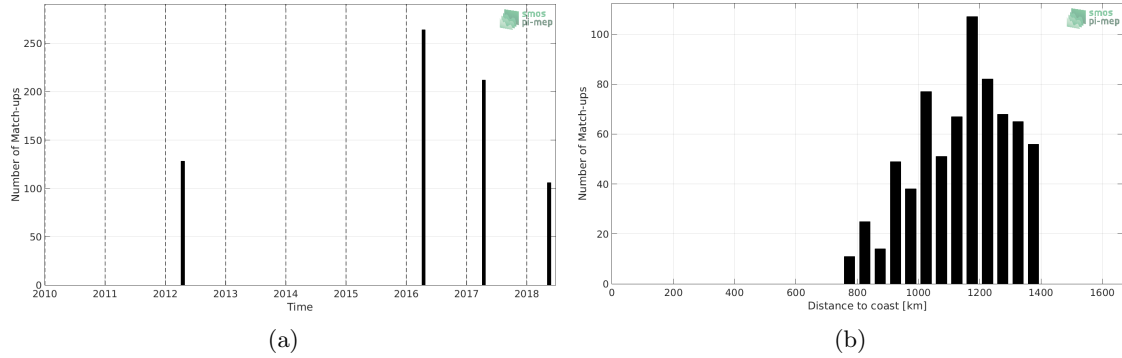
Figure 1: Number of match-ups between TSG-POLARSTERN and CCI-L4-ESA-MERGED-OI-V1.8-30DAY-RUNNING SSS as a function of time (a) and as function of the distance to coast (b) over the Amazon and Orinoco river plumes Pi-MEP region and for the full satellite product period.
