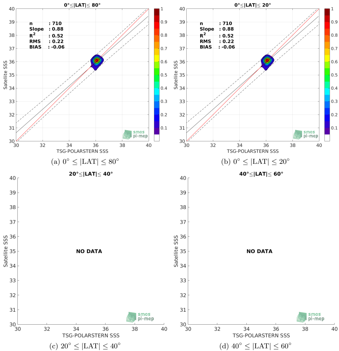
Figure 9: Contour maps of the concentration of CCI-L4-ESA-MERGED-OI-V1.8-30DAY-RUNNING SSS (y-axis) versus TSG-POLARSTERN SSS (x-axis) at match-up pairs for different latitude bands. For each plot, the red line shows x=y . The black thin and dashed lines indicate a linear fit through the data cloud and the \pm 95\% confidence levels, respectively. The number match-up pairs n , the slope and R^2 coefficient of the linear fit, the root mean square (RMS) and the mean bias between satellite and in situ data are indicated for each latitude band in each plots.
