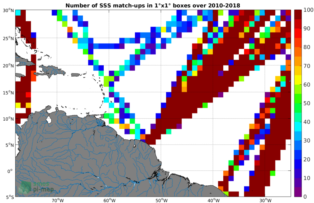
Figure 4: Number of SSS match-ups between TSG-LEGOS-DM SSS and the CCI L4 Merged-OI v1.8 - 30-day running (ESA) SSS product for the Amazon and Orinoco river plumes Pi-MEP region over 1^\circ \times 1^\circ boxes and for the full satellite product period.
