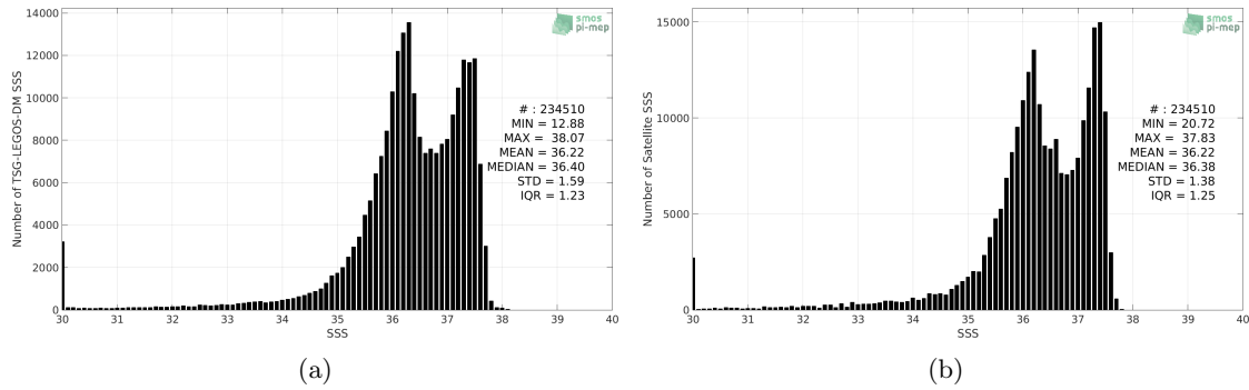
Figure 2: Histograms of SSS from TSG-LEGOS-DM (a) and CCI L4 Merged-OI v1.8 - 30-day running (ESA) (b) considering all match-up pairs per bins of 0.1 over the Amazon and Orinoco river plumes Pi-MEP region and for the full satellite product period.
