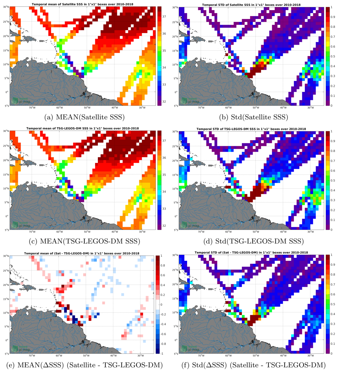
Figure 6: Temporal mean (left) and Std (right) of SSS from CCI L4 Merged-OI v1.8 - 30-day running (ESA) (top), TSG-LEGOS-DM (middle), and of \Delta SSS (Satellite - TSG-LEGOS-DM). Only match-up pairs are used to generate these maps.
