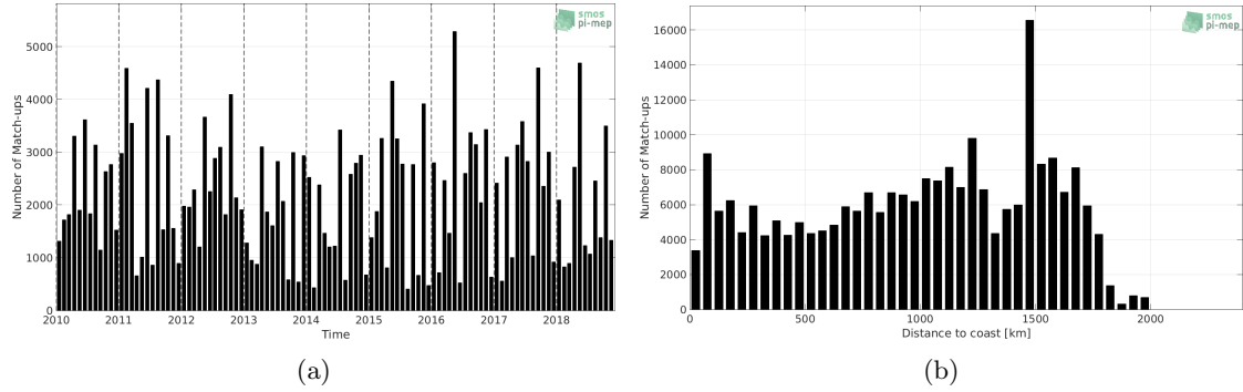
Figure 1: Number of match-ups between TSG-LEGOS-DM and CCI L4 Merged-OI v1.8 - 30-day running (ESA) SSS as a function of time (a) and as function of the distance to coast (b) over the Amazon and Orinoco river plumes Pi-MEP region and for the full satellite product period.
