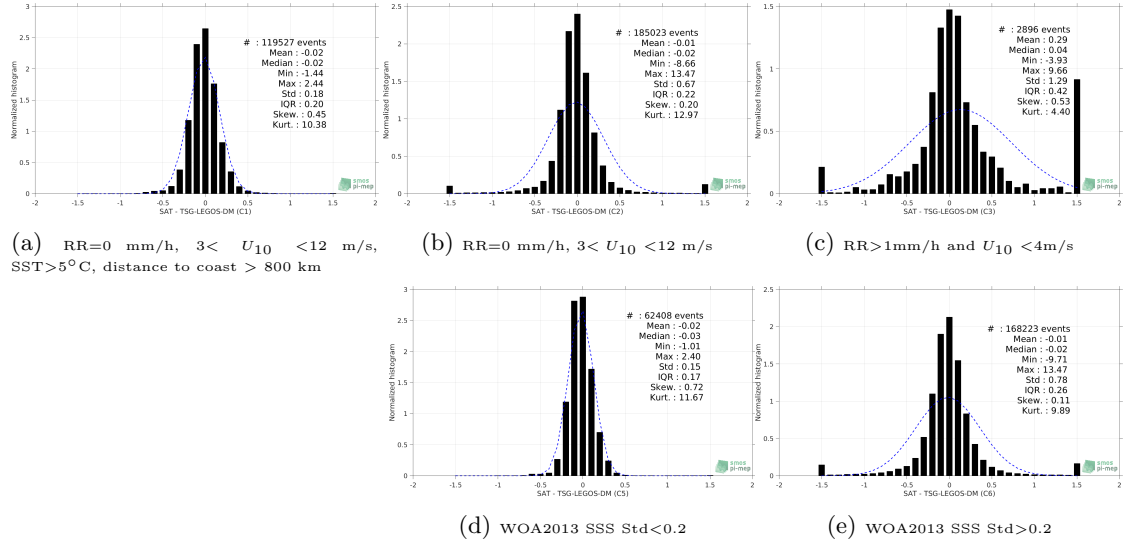
Figure 13: Normalized histogram of \Delta SSS (CCI-L4-ESA-MERGED-OI-V1.8-30DAY-RUNNING - TSG-LEGOS-DM) for 5 different subdatasets corresponding to: RR=0 mm/h, 3 < U_{10} < 12 m/s, SST > 5°C, distance to coast > 800 km (a), RR=0 mm/h, 3 < U_{10} < 12 m/s (b), RR > 1mm/h and U_{10} < 4 m/s (c), WOA2013 SSS Std < 0.2 (d), WOA2013 SSS Std > 0.2 (e).
