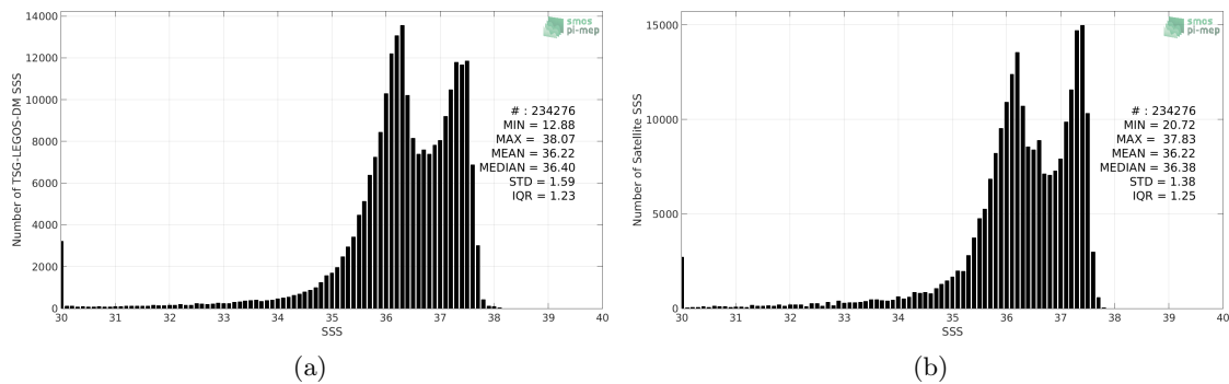
Figure 2: Histograms of SSS from TSG-LEGOS-DM (a) and CCI-L4-ESA-MERGED-OI-V1.8-30DAY-RUNNING (b) considering all match-up pairs per bins of 0.1 over the Amazon and Orinoco river plumes Pi-MEP region and for the full satellite product period.
