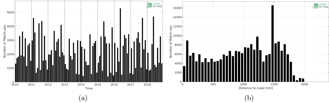
Figure 1: Number of match-ups between TSG-LEGOS-DM and CCI-L4-ESA-MERGED-OI-V1.8-30DAY-RUNNING SSS as a function of time (a) and as function of the distance to coast (b) over the Amazon and Orinoco river plumes Pi-MEP region and for the full satellite product period.
