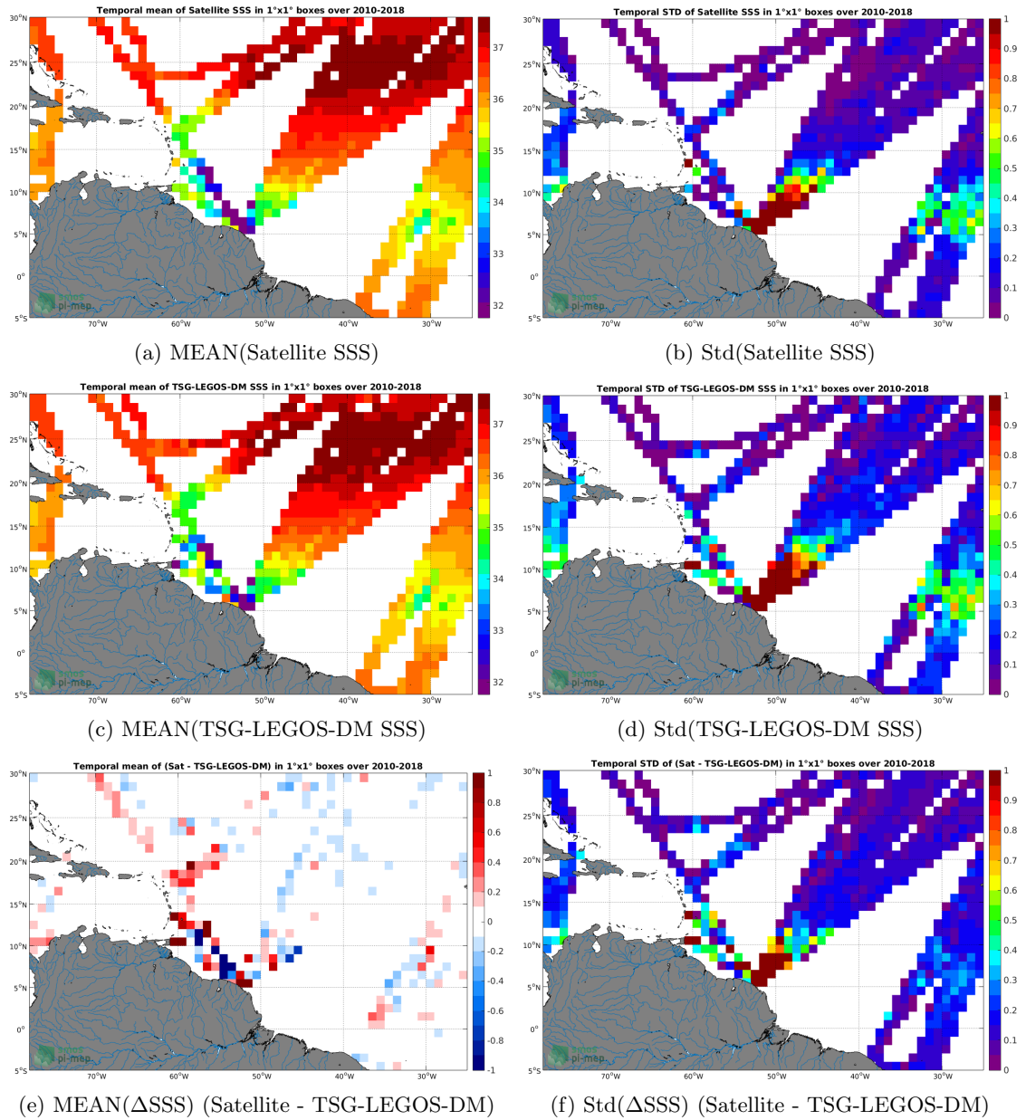
Figure 6: Temporal mean (left) and Std (right) of SSS from CCI-L4-ESA-MERGED-OI-V1.8-30DAY-RUNNING (top), TSG-LEGOS-DM (middle), and of \Delta SSS (Satellite - TSG-LEGOS-DM). Only match-up pairs are used to generate these maps.
