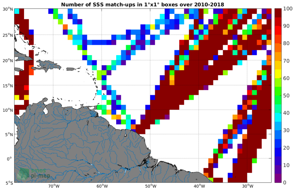
Figure 4: Number of SSS match-ups between TSG-LEGOS-DM SSS and the CCI-L4-ESA-MERGED-OI-V1.8-30DAY-RUNNING SSS product for the Amazon and Orinoco river plumes Pi-MEP region over 1^\circ \times 1^\circ boxes and for the full satellite product period.
