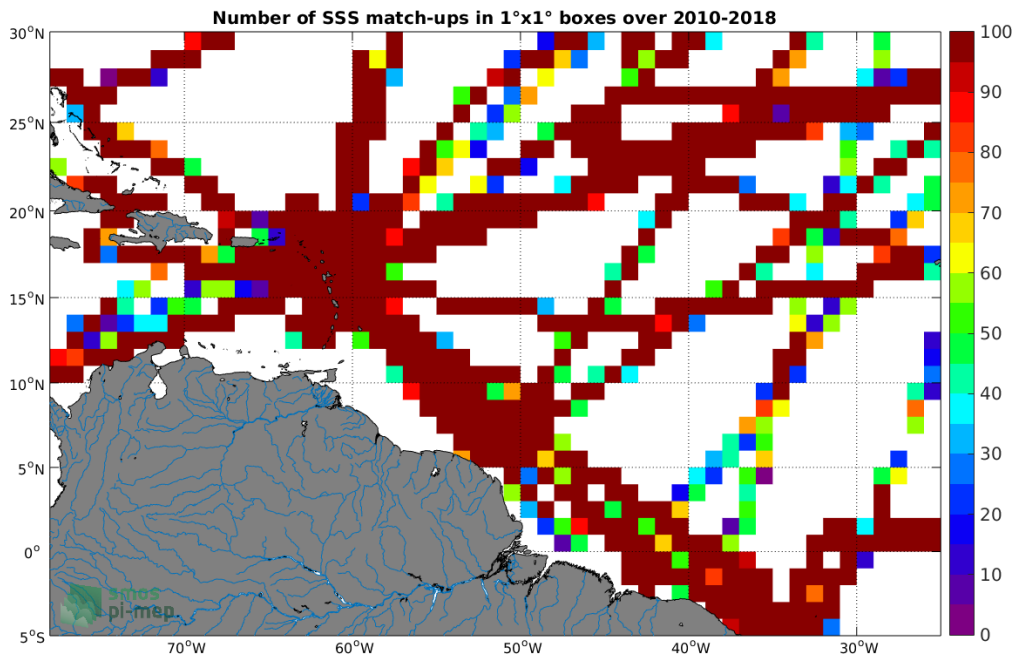
Figure 4: Number of SSS match-ups between TSG-GOSUD-Research-vessel SSS and the CCI L4 Merged-OI v1.8 - 30-day running (ESA) SSS product for the Amazon and Orinoco river plumes Pi-MEP region over 1°x1° boxes and for the full satellite product period.
