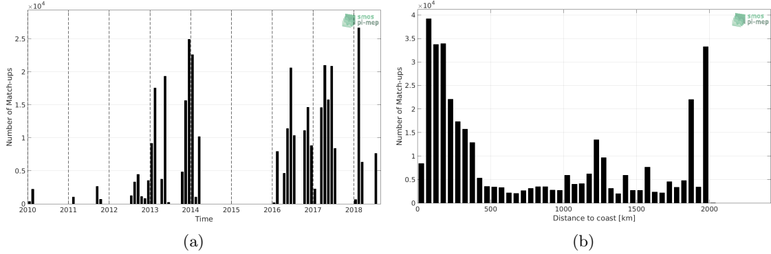
Figure 1: Number of match-ups between TSG-GOSUD-Research-vessel and CCI L4 Merged-OI v1.8 - 30-day running (ESA) SSS as a function of time (a) and as function of the distance to coast (b) over the Amazon and Orinoco river plumes Pi-MEP region and for the full satellite product period.
