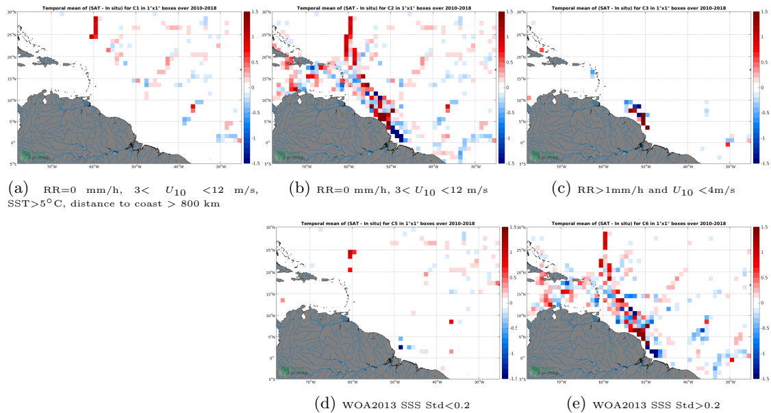
Figure 12: Temporal mean gridded over spatial boxes of size 1^{\circ}\times 1^{\circ} of \Delta SSS (CCI L4 Merged-OI v1.8 - 30-day running (ESA) - TSG-GOSUD-Research-vessel) for 5 different subdatasets corresponding to:RR=0 mm/h, 3 < U_{10} < 12 m/s, SST >5^{\circ}\text{C} , distance to coast > 800 km (a), RR=0 mm/h, 3 < U_{10} < 12 m/s (b), RR >1 mm/h and U_{10} < 4 m/s (c), WOA2013 SSS Std <0.2 (d), WOA2013 SSS Std >0.2 (e).
