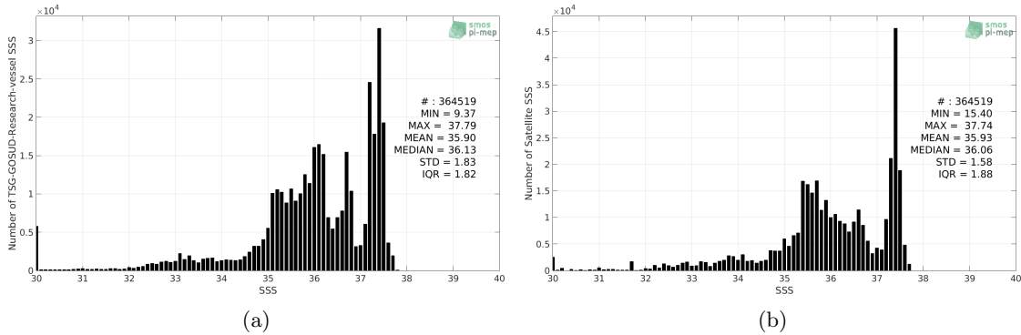
Figure 2: Histograms of SSS from TSG-GOSUD-Research-vessel (a) and CCI L4 Merged-OI v1.8 - 30-day running (ESA) (b) considering all match-up pairs per bins of 0.1 over the Amazon and Orinoco river plumes Pi-MEP region and for the full satellite product period.
