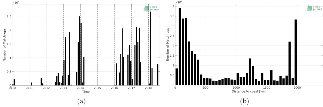
Figure 1: Number of match-ups between TSG-GOSUD-Research-vessel and CCI-L4-ESA-MERGED-OI-V1.8-30DAY-RUNNING SSS as a function of time (a) and as function of the distance to coast (b) over the Amazon and Orinoco river plumes Pi-MEP region and for the full satellite product period.
