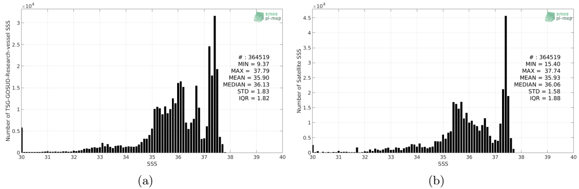
Figure 2: Histograms of SSS from TSG-GOSUD-Research-vessel (a) and CCI-L4-ESA-MERGED-OI-V1.8-30DAY-RUNNING (b) considering all match-up pairs per bins of 0.1 over the Amazon and Orinoco river plumes Pi-MEP region and for the full satellite product period.
