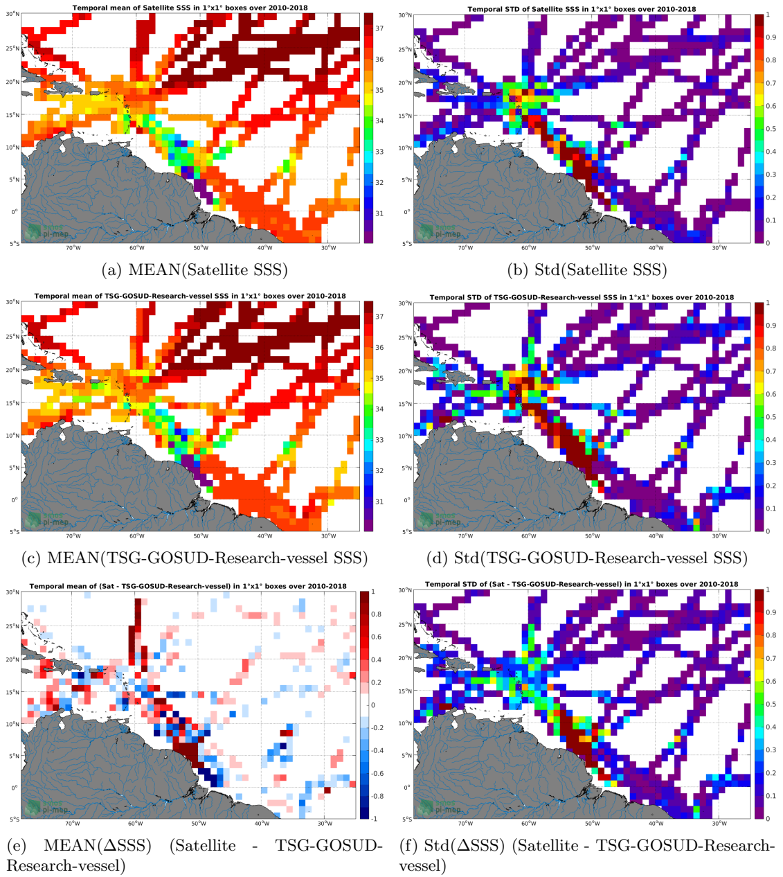
Figure 6: Temporal mean (left) and Std (right) of SSS from CCI-L4-ESA-MERGED-OI-V1.8-30DAY-RUNNING (top), TSG-GOSUD-Research-vessel (middle), and of \Delta SSS (Satellite - TSG-GOSUD-Research-vessel). Only match-up pairs are used to generate these maps.
