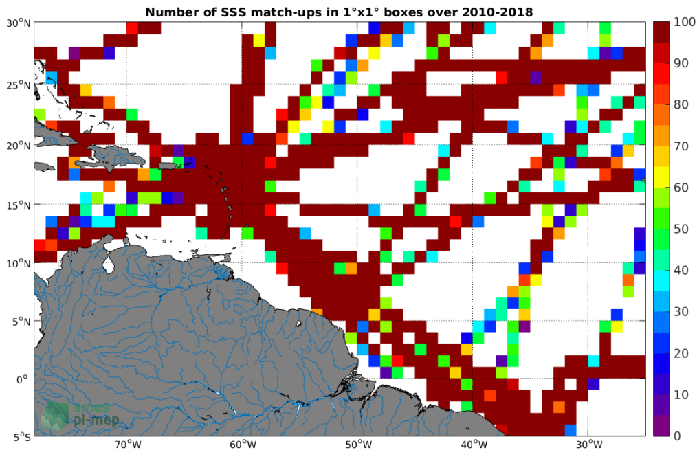
Figure 4: Number of SSS match-ups between TSG-GOSUD-Research-vessel SSS and the CCI-L4-ESA-MERGED-OI-V1.8-30DAY-RUNNING SSS product for the Amazon and Orinoco river plumes Pi-MEP region over 1°x1° boxes and for the full satellite product period.
