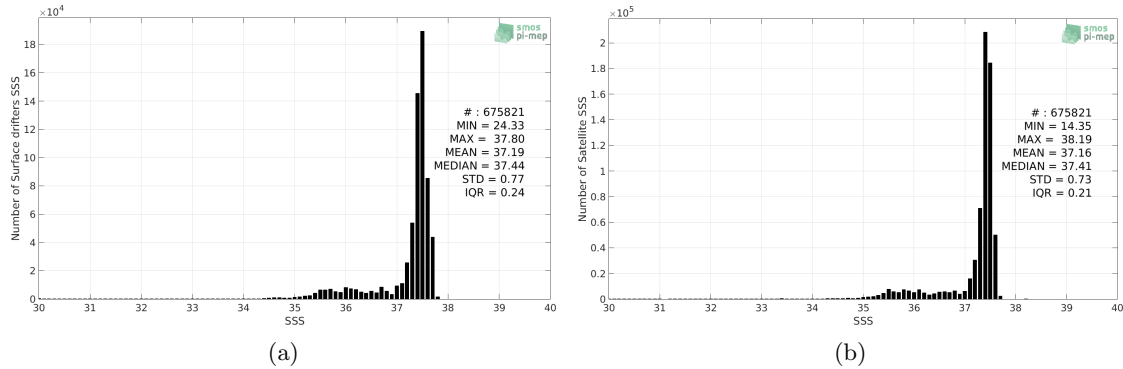
Figure 2: Histograms of SSS from Surface drifters (a) and CCI L4 Merged-OI v1.8 - 30-day running (ESA) (b) considering all match-up pairs per bins of 0.1 over the Amazon and Orinoco river plumes Pi-MEP region and for the full satellite product period.
