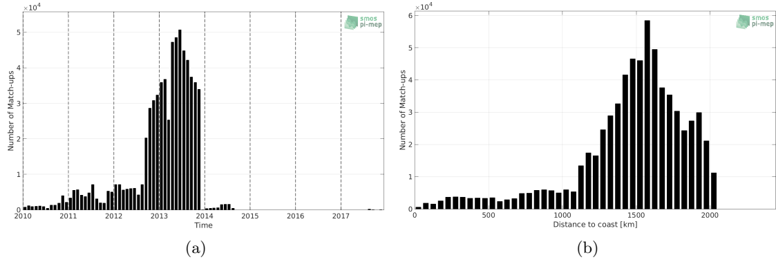
Figure 1: Number of match-ups between Surface drifters and CCI L4 Merged-OI v1.8 - 30-day running (ESA) SSS as a function of time (a) and as function of the distance to coast (b) over the Amazon and Orinoco river plumes Pi-MEP region and for the full satellite product period.
