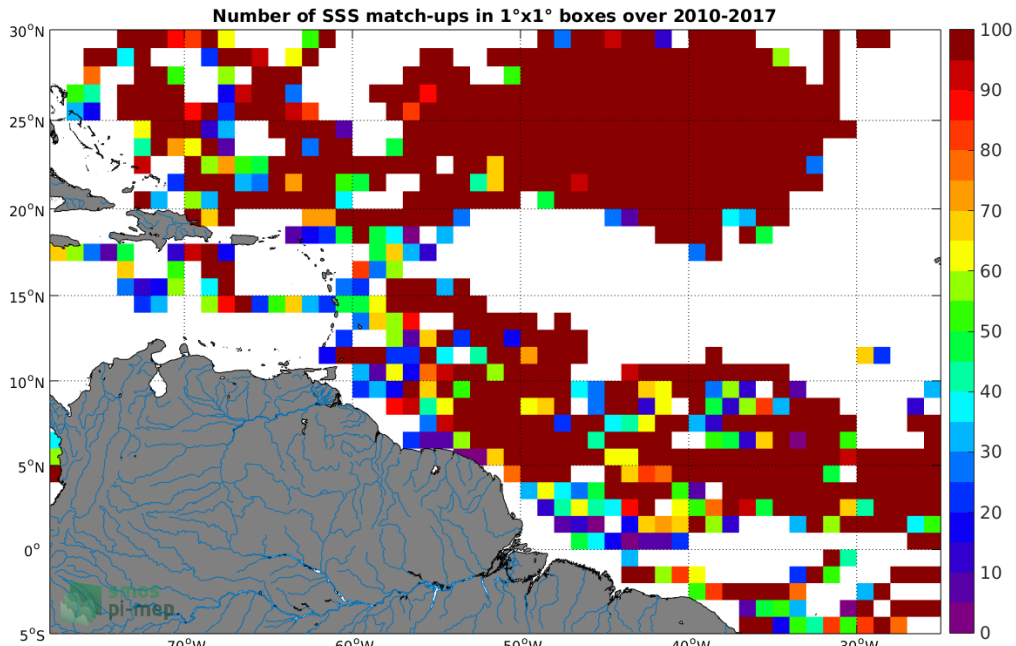
Figure 3: Number of SSS match-ups between Surface drifters SSS and the CCI L4 Merged-OI v1.8 - 30-day running (ESA) SSS product for the Amazon and Orinoco river plumes Pi-MEP region over 1°x1° boxes and for the full satellite product period.
