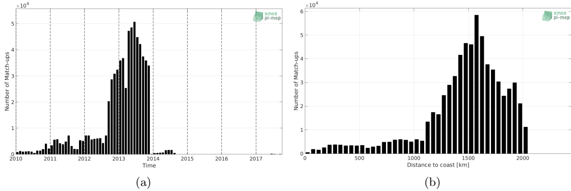
Figure 1: Number of match-ups between Surface drifters and CCI-L4-ESA-MERGED-OI-V1.8-30DAY-RUNNING SSS as a function of time (a) and as function of the distance to coast (b) over the Amazon and Orinoco river plumes Pi-MEP region and for the full satellite product period.
