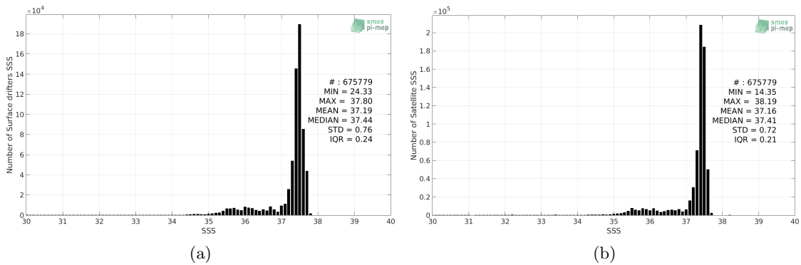
Figure 2: Histograms of SSS from Surface drifters (a) and CCI-L4-ESA-MERGED-OI-V1.8-30DAY-RUNNING (b) considering all match-up pairs per bins of 0.1 over the Amazon and Orinoco river plumes Pi-MEP region and for the full satellite product period.
