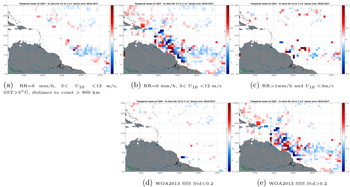
Figure 11: Temporal mean gridded over spatial boxes of size 1^\circ \times 1^\circ of \Delta SSS (CCI-L4-ESAMERGED-OI-V1.8-30DAY-RUNNING - Surface drifters) for 5 different subdatasets corresponding to:RR=0 mm/h, 3 < U_{10} < 12 m/s, SST >5^\circ\text{C} , distance to coast > 800 km (a), RR=0 mm/h, 3 < U_{10} < 12 m/s (b), RR >1 mm/h and U_{10} < 4 m/s (c), WOA2013 SSS Std <0.2 (d), WOA2013 SSS Std >0.2 (e).
