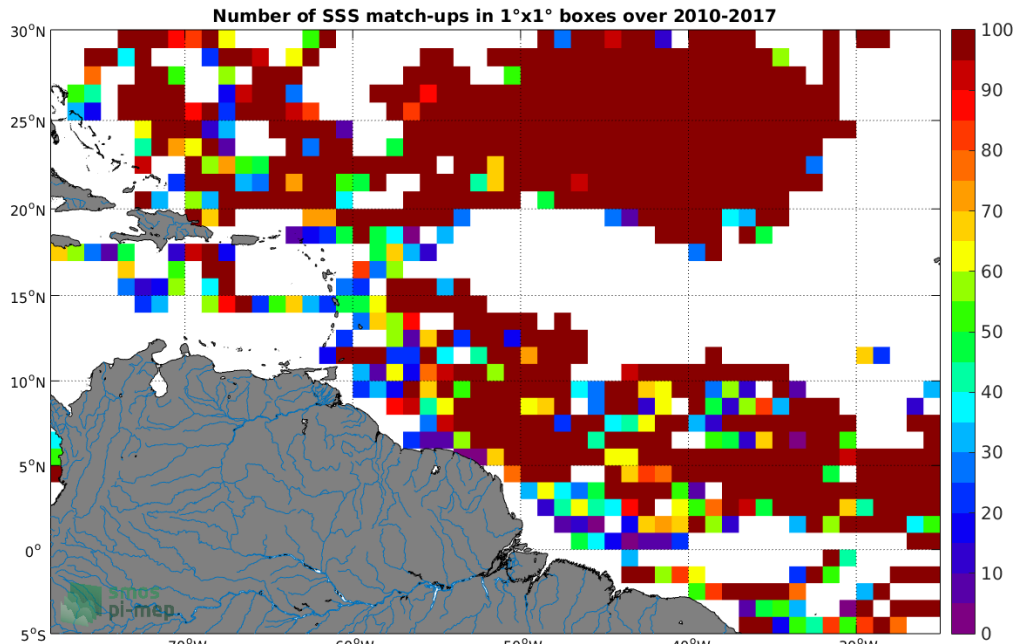
Figure 3: Number of SSS match-ups between Surface drifters SSS and the CCI-L4-ESA-MERGED-OI-V1.8-30DAY-RUNNING SSS product for the Amazon and Orinoco river plumes Pi-MEP region over 1^{\circ} \times 1^{\circ} boxes and for the full satellite product period.
