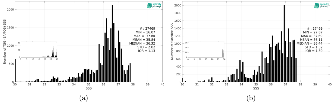
Figure 3: Histograms of SSS from TSG (SAMOS) (a) and Aquarius SSS L4 OI v5 - Weekly (IPRC) (b) considering all match-up pairs per bins of 0.1 over the Amazon and Orinoco river plumes Pi-MEP region and for the full satellite product period.
