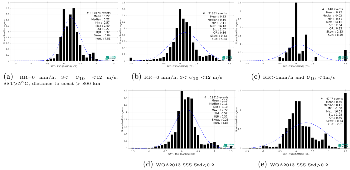
Figure 15: Normalized histogram of \Delta\text{SSS} (Aquarius SSS L4 OI v5 - Weekly (IPRC) - TSG (SAMOS)) for 5 different subdatasets corresponding to: RR=0 mm/h, 3 < U_{10} < 12 m/s, SST>5°C, distance to coast > 800 km (a), RR=0 mm/h, 3 < U_{10} < 12 m/s (b), RR>1mm/h and U_{10} < 4 m/s (c), WOA2013 SSS Std<0.2 (d), WOA2013 SSS Std>0.2 (e).
