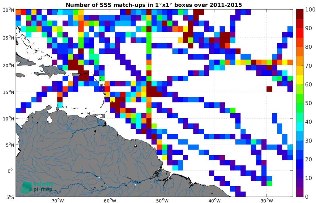
Figure 5: Number of SSS match-ups between TSG (SAMOS) SSS and the Aquarius SSS L4 OI v5 - Weekly (IPRC) SSS product for the Amazon and Orinoco river plumes Pi-MEP region over 1^\circ \times 1^\circ boxes and for the full satellite product period.
