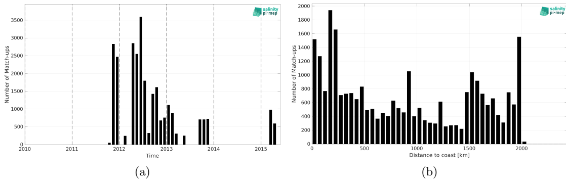
Figure 2: Number of match-ups between TSG (SAMOS) and Aquarius SSS L4 OI v5 - Weekly (IPRC) SSS as a function of time (a) and as function of the distance to coast (b) over the Amazon and Orinoco river plumes Pi-MEP region and for the full satellite product period.
