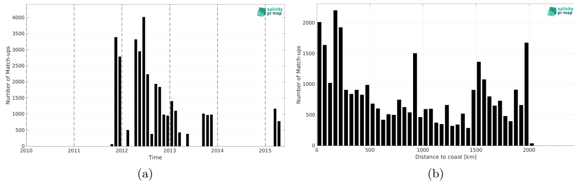
Figure 1: Number of match-ups between TSG (SAMOS) and Aquarius SSS L4 OI v5 - Weekly (IPRC) SSS as a function of time (a) and as function of the distance to coast (b) over the Amazon and Orinoco river plumes Pi-MEP region and for the full satellite product period.
