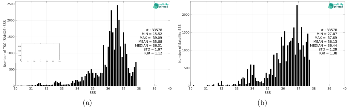
Figure 2: Histograms of SSS from TSG (SAMOS) (a) and Aquarius SSS L4 OI v5 - Weekly (IPRC) (b) considering all match-up pairs per bins of 0.1 over the Amazon and Orinoco river plumes Pi-MEP region and for the full satellite product period.
