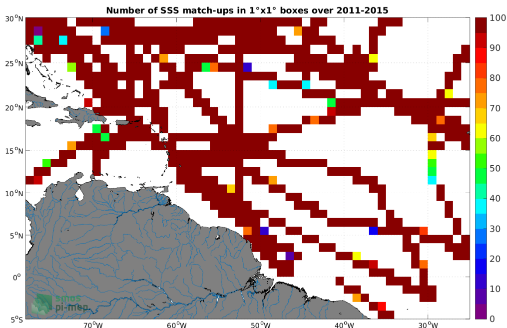
Figure 4: Number of SSS match-ups between TSG (SAMOS) SSS and the Aquarius SSS L4 OI v5 - Weekly (IPRC) SSS product for the Amazon and Orinoco river plumes Pi-MEP region over 1°×1° boxes and for the full satellite product period.
