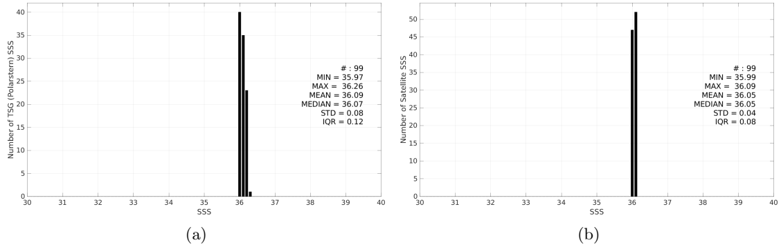
Figure 3: Histograms of SSS from TSG (Polarstern) (a) and Aquarius SSS L4 OI v5 - Weekly (IPRC) (b) considering all match-up pairs per bins of 0.1 over the Amazon and Orinoco river plumes Pi-MEP region and for the full satellite product period.
