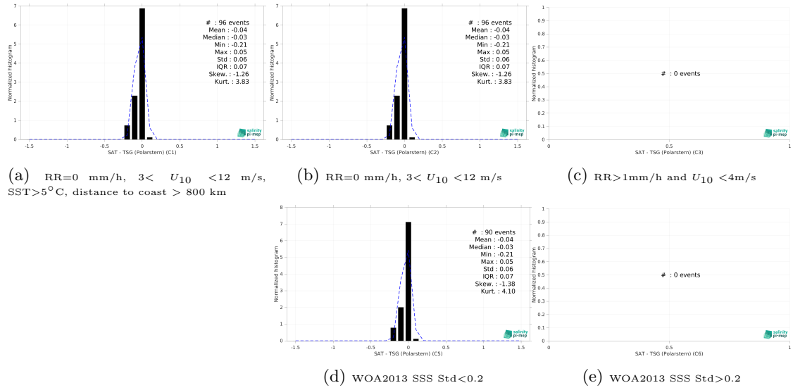
Figure 15: Normalized histogram of \Delta\text{SSS} (Aquarius SSS L4 OI v5 - Weekly (IPRC) - TSG (Polarstern)) for 5 different subdatasets corresponding to: RR=0 mm/h, 3 < U_{10} < 12 m/s, SST > 5^\circ\text{C} , distance to coast > 800 km (a), RR=0 mm/h, 3 < U_{10} < 12 m/s (b), RR > 1\text{mm/h} and U_{10} < 4\text{m/s} (c), WOA2013 SSS Std < 0.2 (d), WOA2013 SSS Std > 0.2 (e).
