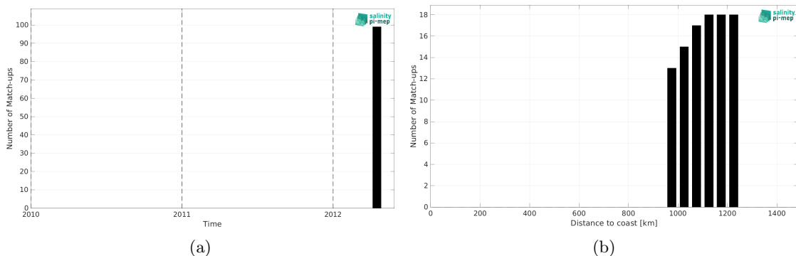
Figure 2: Number of match-ups between TSG (Polarstern) and Aquarius SSS L4 OI v5 - Weekly (IPRC) SSS as a function of time (a) and as function of the distance to coast (b) over the Amazon and Orinoco river plumes Pi-MEP region and for the full satellite product period.
