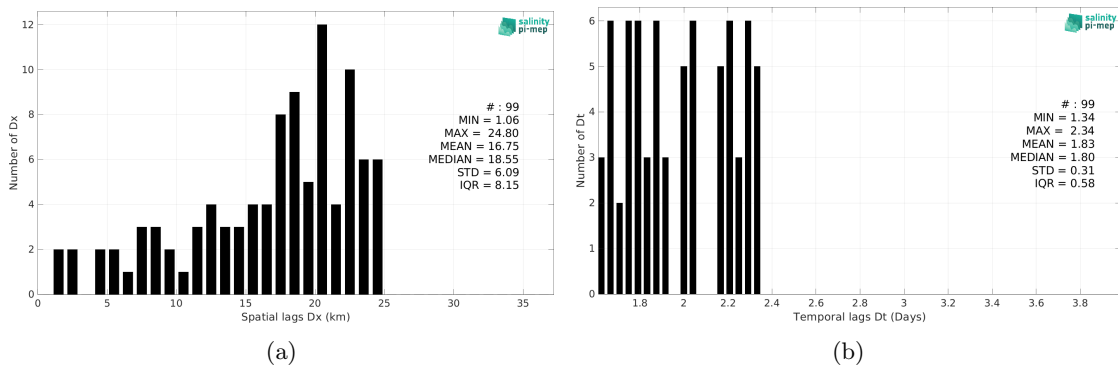
Figure 6: Histograms of the spatial (a) and temporal (b) lags between the location/time of the TSG (Polarstern) measurement and the date of the corresponding Aquarius SSS L4 OI v5 - Weekly (IPRC) SSS pixel.
