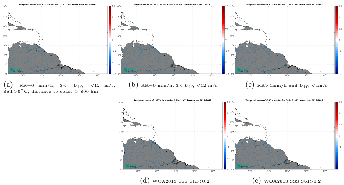
Figure 14: Temporal mean gridded over spatial boxes of size 1^\circ \times 1^\circ of \Delta SSS (Aquarius SSS L4 OI v5 - Weekly (IPRC) - TSG (Polarstern)) for 5 different subdatasets corresponding to:RR=0 mm/h, 3 < U_{10} < 12 m/s, SST >5^\circ\text{C} , distance to coast > 800 km (a), RR=0 mm/h, 3 < U_{10} < 12 m/s (b), RR >1 mm/h and U_{10} < 4 m/s (c), WOA2013 SSS Std <0.2 (d), WOA2013 SSS Std >0.2 (e).
