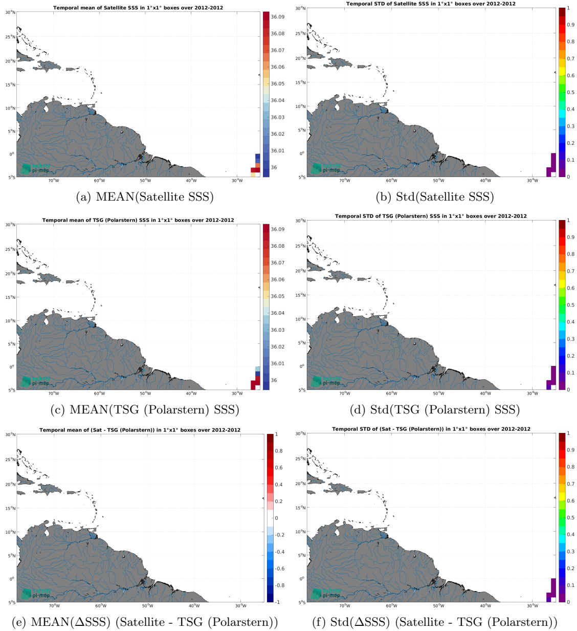
Figure 7: Temporal mean (left) and Std (right) of SSS from Aquarius SSS L4 OI v5 - Weekly (IPRC) (top), TSG (Polarstern) (middle), and of \Delta SSS (Satellite - TSG (Polarstern)). Only match-up pairs are used to generate these maps.
