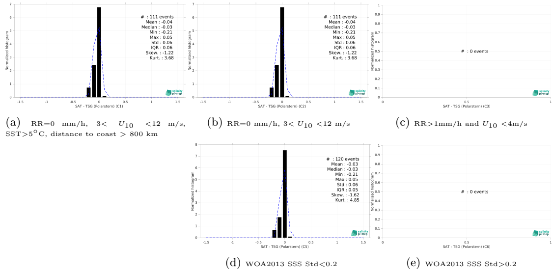
Figure 13: Normalized histogram of \Delta\text{SSS} (Aquarius SSS L4 OI v5 - Weekly (IPRC) - TSG (Polarstern)) for 5 different subdatasets corresponding to: RR=0 mm/h, 3 < U_{10} < 12 m/s, SST >5^{\circ}\text{C} , distance to coast > 800 km (a), RR=0 mm/h, 3 < U_{10} < 12 m/s (b), RR >1 mm/h and U_{10} < 4 m/s (c), WOA2013 SSS Std <0.2 (d), WOA2013 SSS Std >0.2 (e).
