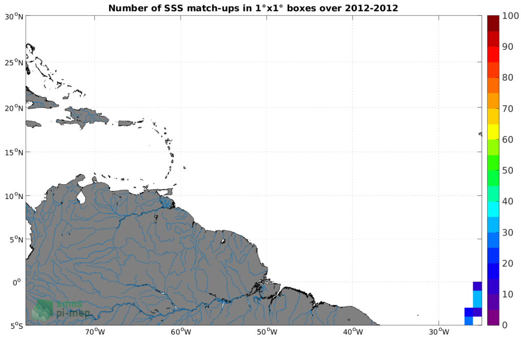
Figure 4: Number of SSS match-ups between TSG (Polarstern) SSS and the Aquarius SSS L4 OI v5 - Weekly (IPRC) SSS product for the Amazon and Orinoco river plumes Pi-MEP region over 1°×1° boxes and for the full satellite product period.
