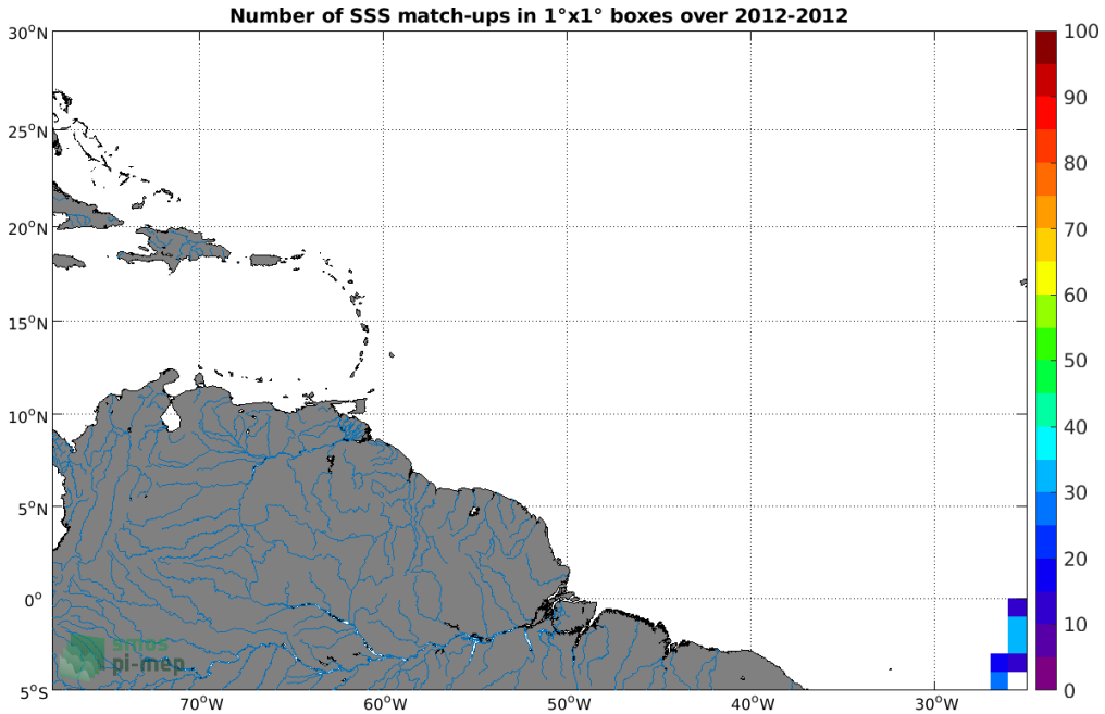
Figure 4: Number of SSS match-ups between TSG (Polarstern) SSS and the Aquarius SSS L4 OI v5 - Weekly (IPRC) SSS product for the Amazon and Orinoco river plumes Pi-MEP region over 1^{\circ} \times 1^{\circ} boxes and for the full satellite product period.
