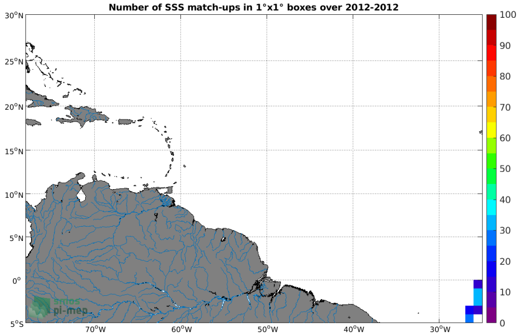
Figure 4: Number of SSS match-ups between TSG (Polarstern) SSS and the Aquarius SSS L4 OI v5 - Weekly (IPRC) SSS product for the Amazon and Orinoco river plumes Pi-MEP region over 1°x1° boxes and for the full satellite product period.
