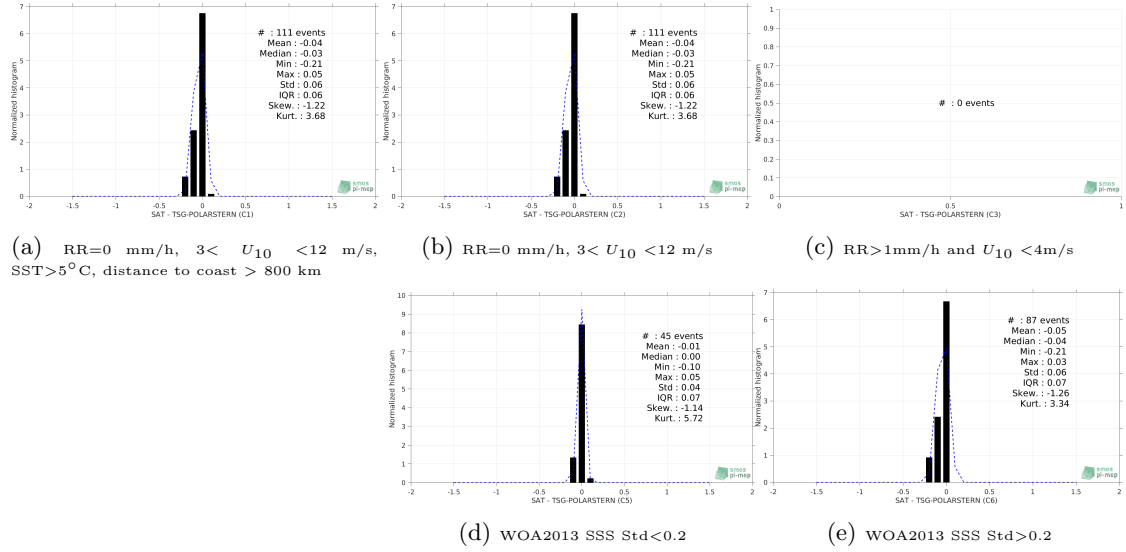
Figure 13: Normalized histogram of \Delta SSS (Aquarius-L4-IPRC-V5-WEEKLY - TSG-POLARSTERN) for 5 different subdatasets corresponding to: RR=0 mm/h, 3 < U_{10} < 12 m/s, SST > 5°C, distance to coast > 800 km (a), RR=0 mm/h, 3 < U_{10} < 12 m/s (b), RR > 1mm/h and U_{10} < 4 m/s (c), WOA2013 SSS Std < 0.2 (d), WOA2013 SSS Std > 0.2 (e).
