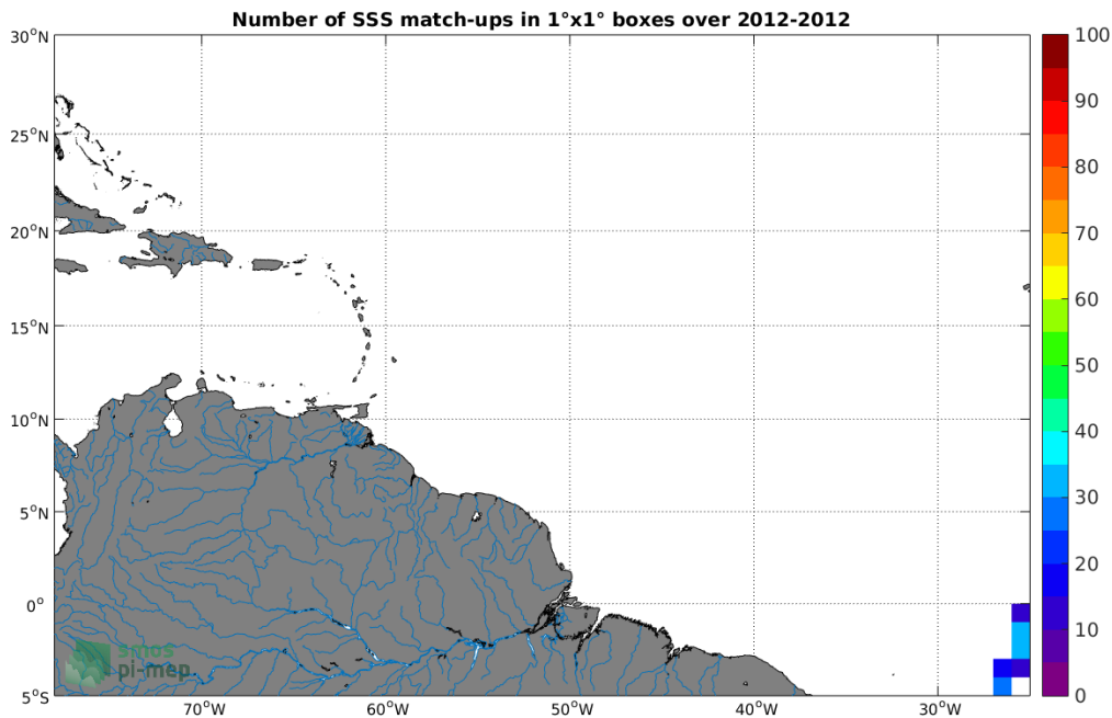
Figure 4: Number of SSS match-ups between TSG-POLARSTERN SSS and the Aquarius-L4-IPRC-V5-WEEKLY SSS product for the Amazon and Orinoco river plumes Pi-MEP region over 1^\circ \times 1^\circ boxes and for the full satellite product period.
