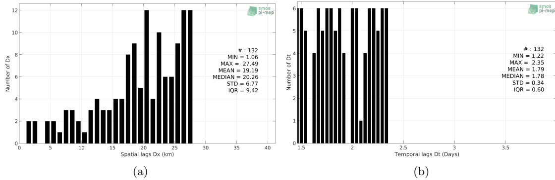
Figure 5: Histograms of the spatial (a) and temporal (b) lags between the time of the TSG-POLARSTERN measurements and the date of the corresponding Aquarius-L4-IPRC-V5-WEEKLY SSS product.
