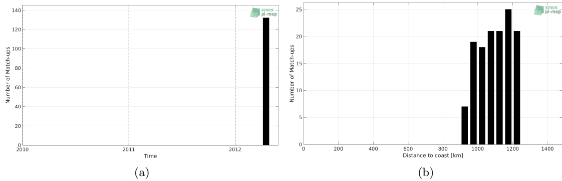
Figure 1: Number of match-ups between TSG-POLARSTERN and Aquarius-L4-IPRC-V5-WEEKLY SSS as a function of time (a) and as function of the distance to coast (b) over the Amazon and Orinoco river plumes Pi-MEP region and for the full satellite product period.
