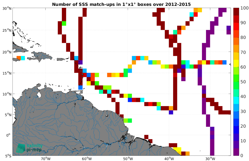
Figure 5: Number of SSS match-ups between TSG (GOSUD-Sailing-ship) SSS and the Aquarius SSS L4 OI v5 - Weekly (IPRC) SSS product for the Amazon and Orinoco river plumes Pi-MEP region over 1^\circ \times 1^\circ boxes and for the full satellite product period.
