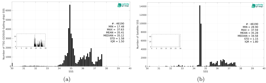
Figure 3: Histograms of SSS from TSG (GOSUD-Sailing-ship) (a) and Aquarius SSS L4 OI v5 - Weekly (IPRC) (b) considering all match-up pairs per bins of 0.1 over the Amazon and Orinoco river plumes Pi-MEP region and for the full satellite product period.
