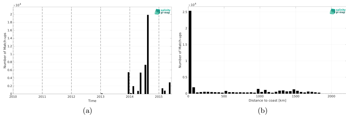
Figure 2: Number of match-ups between TSG (GOSUD-Sailing-ship) and Aquarius SSS L4 OI v5 - Weekly (IPRC) SSS as a function of time (a) and as function of the distance to coast (b) over the Amazon and Orinoco river plumes Pi-MEP region and for the full satellite product period.
