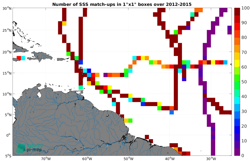
Figure 4: Number of SSS match-ups between TSG (GOSUD-Sailing-ship) SSS and the Aquarius SSS L4 OI v5 - Weekly (IPRC) SSS product for the Amazon and Orinoco river plumes Pi-MEP region over 1^{\circ} \times 1^{\circ} boxes and for the full satellite product period.
