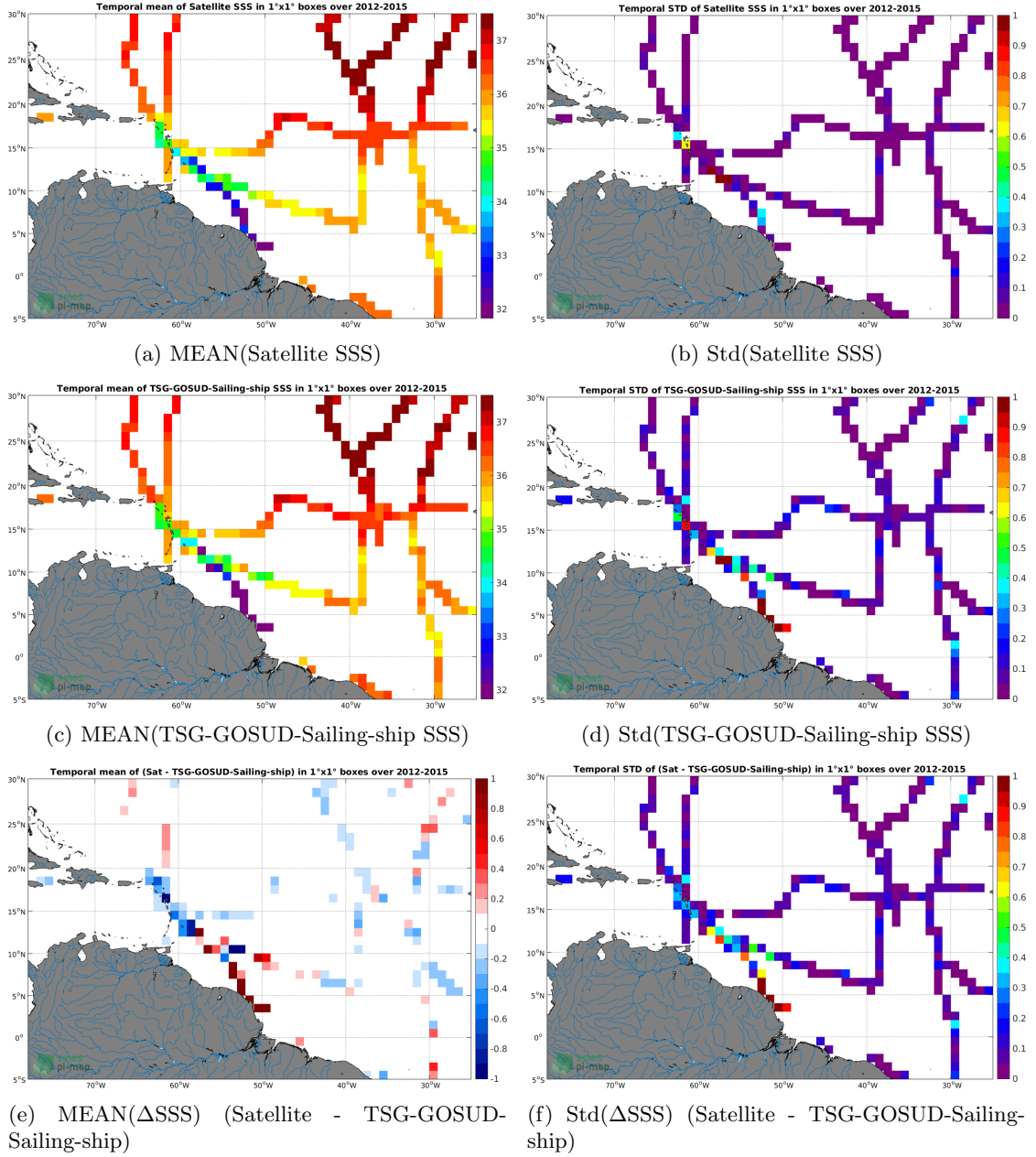
Figure 6: Temporal mean (left) and Std (right) of SSS from Aquarius-L4-IPRC-V5-WEEKLY (top), TSG-GOSUD-Sailing-ship (middle), and of \Delta SSS (Satellite - TSG-GOSUD-Sailing-ship). Only match-up pairs are used to generate these maps.
