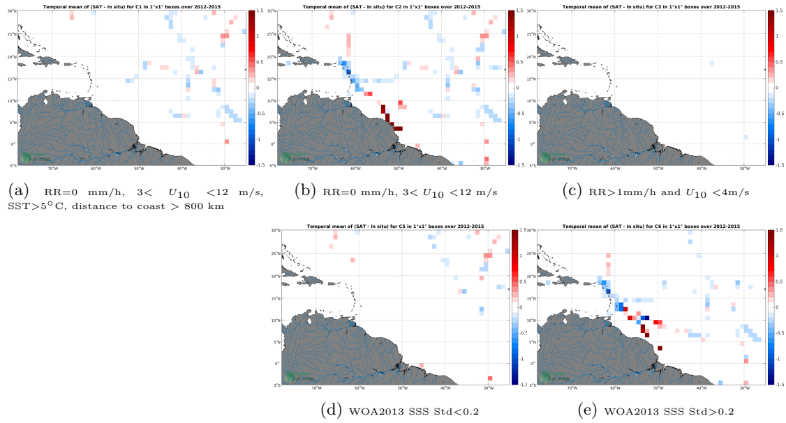
Figure 12: Temporal mean gridded over spatial boxes of size 1^\circ \times 1^\circ of \Delta SSS (Aquarius-L4-IPRC-V5-WEEKLY - TSG-GOSUD-Sailing-ship) for 5 different subdatasets corresponding to: RR=0 mm/h, 3 < U_{10} < 12 m/s, SST > 5^\circ C , distance to coast > 800 km (a), RR=0 mm/h, 3 < U_{10} < 12 m/s (b), RR > 1 mm/h and U_{10} < 4 m/s (c), WOA2013 SSS Std < 0.2 (d), WOA2013 SSS Std > 0.2 (e).
