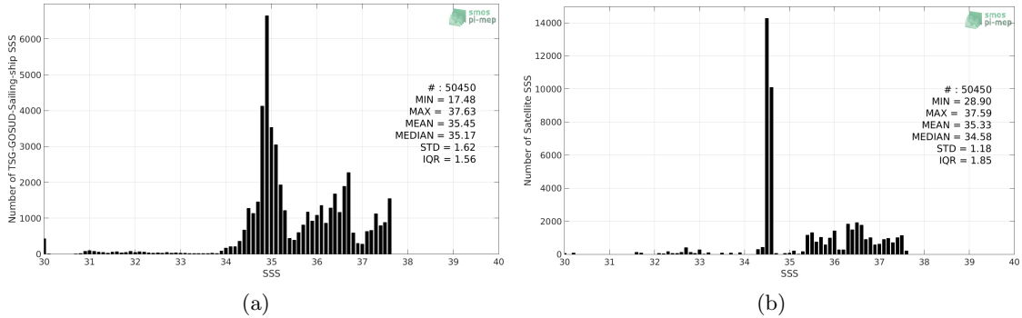
Figure 2: Histograms of SSS from TSG-GOSUD-Sailing-ship (a) and Aquarius-L4-IPRC-V5-WEEKLY (b) considering all match-up pairs per bins of 0.1 over the Amazon and Orinoco river plumes Pi-MEP region and for the full satellite product period.
