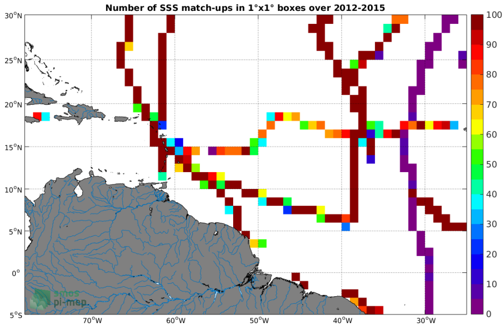
Figure 4: Number of SSS match-ups between TSG-GOSUD-Sailing-ship SSS and the Aquarius-L4-IPRC-V5-WEEKLY SSS product for the Amazon and Orinoco river plumes Pi-MEP region over 1^\circ \times 1^\circ boxes and for the full satellite product period.
