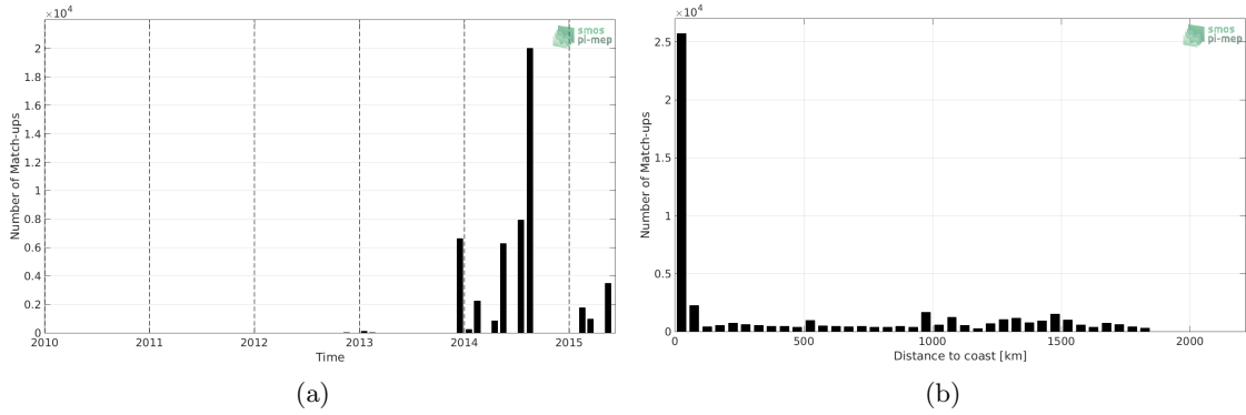
Figure 1: Number of match-ups between TSG-GOSUD-Sailing-ship and Aquarius-L4-IPRC-V5-WEEKLY SSS as a function of time (a) and as function of the distance to coast (b) over the Amazon and Orinoco river plumes Pi-MEP region and for the full satellite product period.
