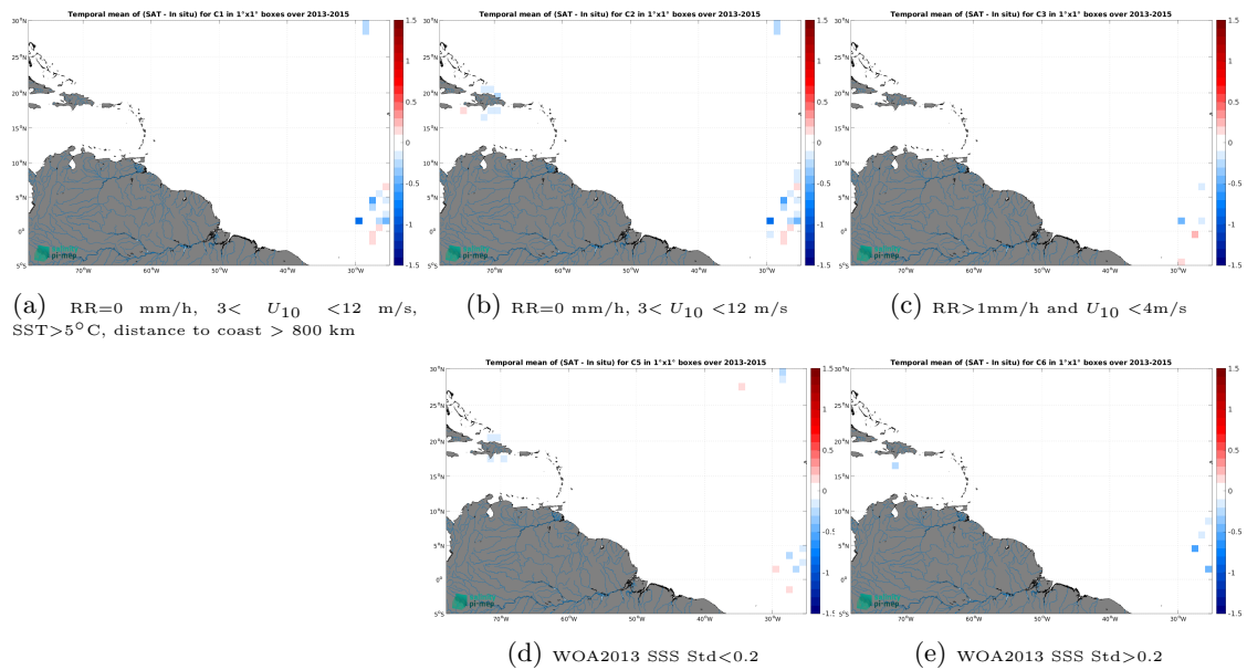
Figure 14: Temporal mean gridded over spatial boxes of size 1^\circ \times 1^\circ of \Delta SSS (Aquarius SSS L4 OI v5 - Weekly (IPRC) - TSG (CSIC-UTM)) for 5 different subdatasets corresponding to:RR=0 mm/h, 3 < U_{10} < 12 m/s, SST >5^\circ\text{C} , distance to coast > 800 km (a), RR=0 mm/h, 3 < U_{10} < 12 m/s (b), RR >1 mm/h and U_{10} < 4 m/s (c), WOA2013 SSS Std <0.2 (d), WOA2013 SSS Std >0.2 (e).
