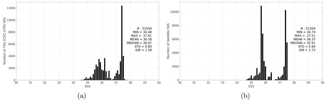
Figure 3: Histograms of SSS from TSG (CSIC-UTM) (a) and Aquarius SSS L4 OI v5 - Weekly (IPRC) (b) considering all match-up pairs per bins of 0.1 over the Amazon and Orinoco river plumes Pi-MEP region and for the full satellite product period.
