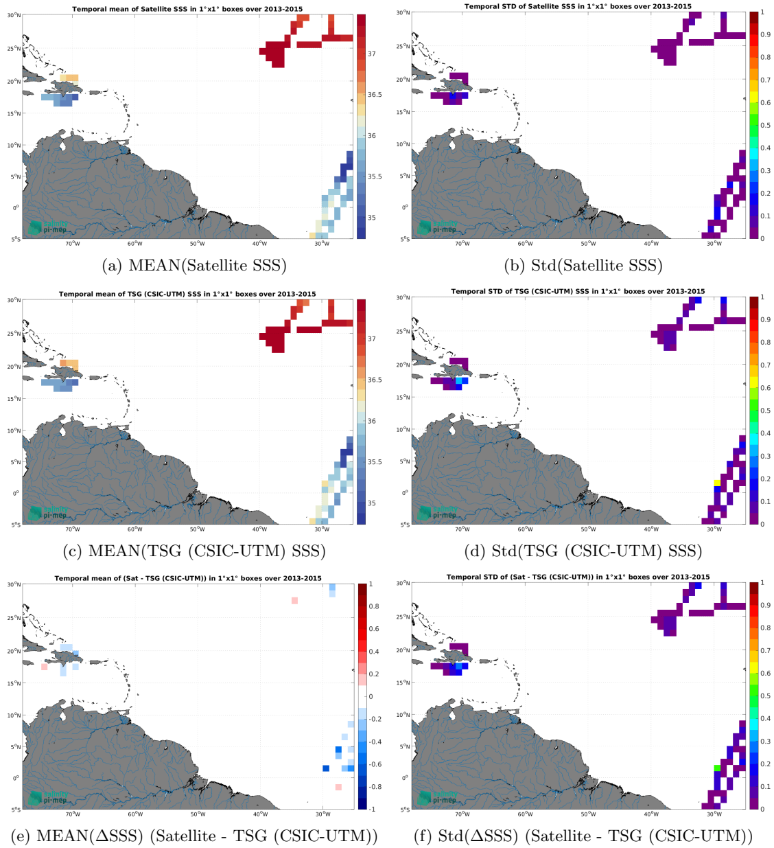
Figure 7: Temporal mean (left) and Std (right) of SSS from Aquarius SSS L4 OI v5 - Weekly (IPRC) (top), TSG (CSIC-UTM) (middle), and of \Delta SSS (Satellite - TSG (CSIC-UTM)). Only match-up pairs are used to generate these maps.
