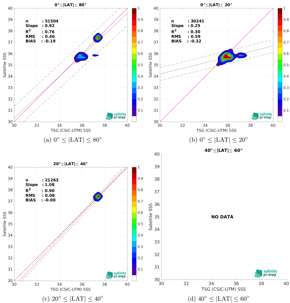
Figure 10: Contour maps of the concentration of Aquarius SSS L4 OI v5 - Weekly (IPRC) SSS (y-axis) versus TSG (CSIC-UTM) SSS (x-axis) at match-up pairs for different latitude bands. For each plot, the red line shows x=y . The black thin and dashed lines indicate a linear fit through the data cloud and the \pm 95\% confidence levels, respectively. The number match-up pairs n , the slope and R^2 coefficient of the linear fit, the root mean square (RMS) and the mean bias between satellite and in situ data are indicated for each latitude band in each plots.
