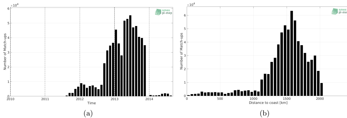
Figure 1: Number of match-ups between Surface drifters and Aquarius SSS L4 OI v5 - Weekly (IPRC) SSS as a function of time (a) and as function of the distance to coast (b) over the Amazon and Orinoco river plumes Pi-MEP region and for the full satellite product period.
