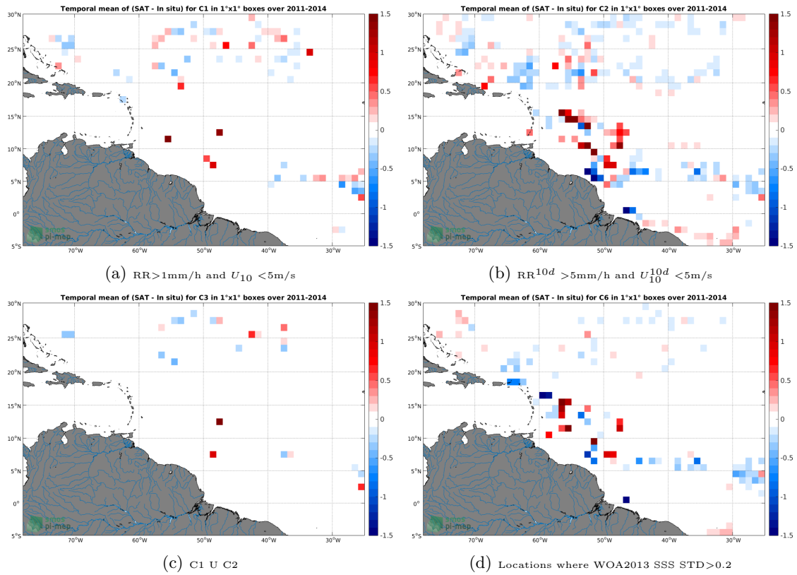
Figure 11: Temporal mean gridded over spatial boxes of size 1^\circ \times 1^\circ of \Delta SSS (Aquarius-L4-IPRC-V5-WEEKLY - Surface drifters) for 4 different subdatasets corresponding to: RR > 1\text{mm/h} and U_{10} < 5\text{m/s} (a), RR^{10d} > 5\text{mm/h} and U_{10}^{10d} < 5\text{m/s} (b), C1 U C2 (c), Locations where WOA2013 SSS STD > 0.2 (d).
