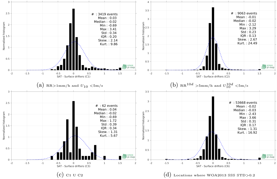
Figure 12: Normalized histogram of \Delta SSS (Aquarius-L4-IPRC-V5-WEEKLY - Surface drifters) for 6 different subdatasets corresponding to: RR > 1mm/h and U_{10} < 5 m/s (a), RR^{10d} > 5 mm/h and U_{10}^{10d} < 5 m/s (b), C1 U C2 (c), Locations where WOA2013 SSS STD > 0.2 (d).
