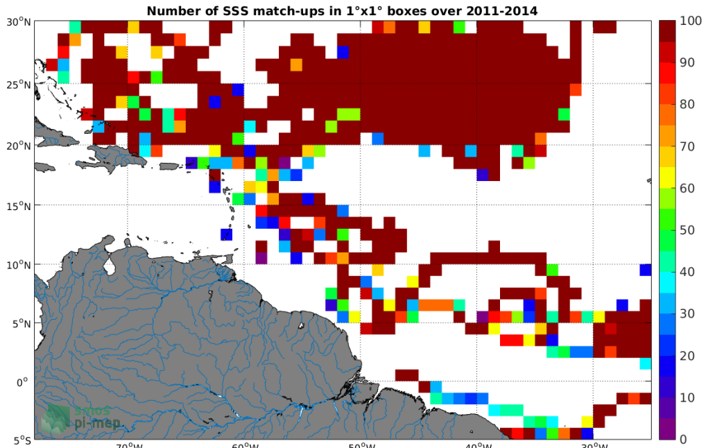
Figure 3: Number of SSS match-ups between Surface drifters SSS and the Aquarius-L4-IPRC-V5-WEEKLY SSS product for the Amazon and Orinoco river plumes Pi-MEP region over 1^{\circ} \times 1^{\circ} boxes and for the full satellite product period.
