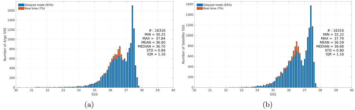
Figure 3: Histograms of SSS from Argo (a) and Aquarius SSS L4 OI v5 - Weekly (IPRC) (b) considering all match-up pairs per bins of 0.1 over the Amazon and Orinoco river plumes Pi-MEP region and for the full satellite product period.
