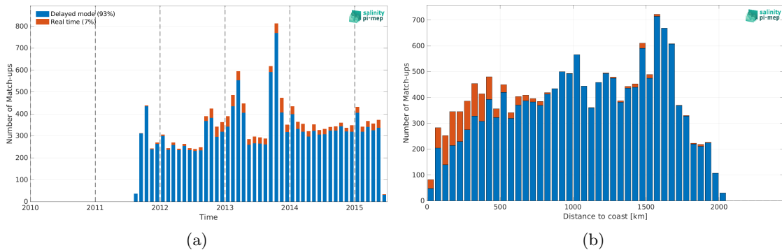
Figure 2: Number of match-ups between Argo and Aquarius SSS L4 OI v5 - Weekly (IPRC) SSS as a function of time (a) and as function of the distance to coast (b) over the Amazon and Orinoco river plumes Pi-MEP region and for the full satellite product period.
