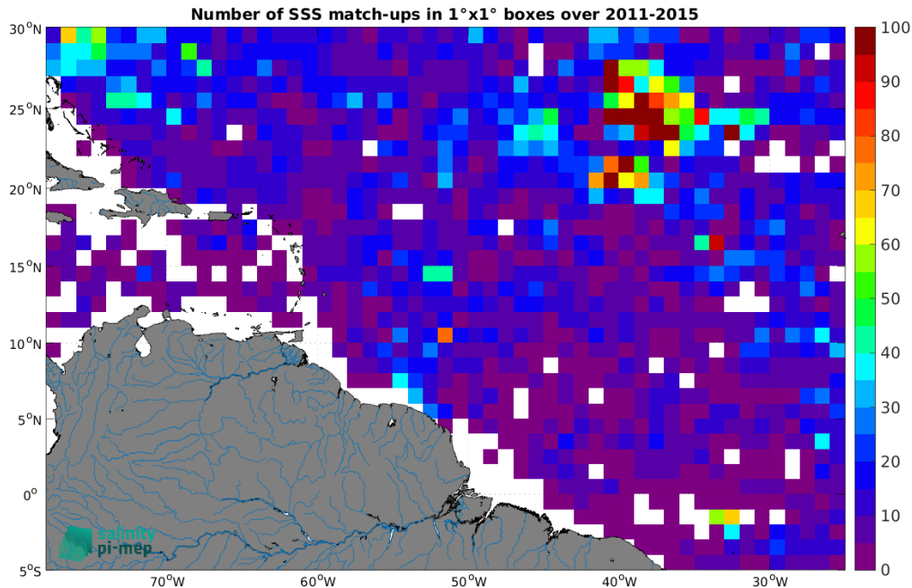
Figure 5: Number of SSS match-ups between Argo SSS and the Aquarius SSS L4 OI v5 - Weekly (IPRC) SSS product for the Amazon and Orinoco river plumes Pi-MEP region over 1^\circ \times 1^\circ boxes and for the full satellite product period.
