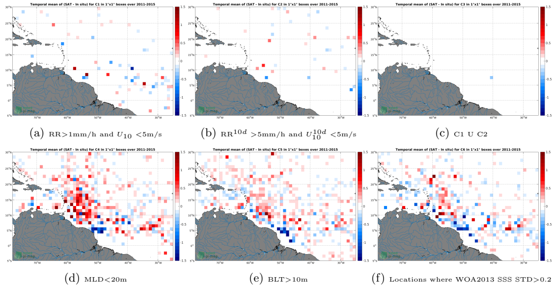
Figure 12: Temporal mean gridded over spatial boxes of size 1^\circ \times 1^\circ of \Delta\text{SSS} (Aquarius-L4-IPRC-V5-WEEKLY - Argo) for 6 different subdatasets corresponding to: \text{RR} > 1\text{mm/h} and U_{10} < 5\text{m/s} (a), \text{RR}^{10d} > 5\text{mm/h} and U_{10}^{10d} < 5\text{m/s} (b), C1 U C2 (c), \text{MLD} < 20\text{m} (d), \text{BLT} > 10\text{m} (e), Locations where WOA2013 SSS STD > 0.2 (f).
