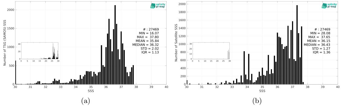
Figure 3: Histograms of SSS from TSG (SAMOS) (a) and Aquarius SSS L4 OI v5 - Monthly (IPRC) (b) considering all match-up pairs per bins of 0.1 over the Amazon and Orinoco river plumes Pi-MEP region and for the full satellite product period.
