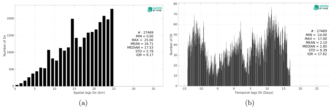
Figure 6: Histograms of the spatial (a) and temporal (b) lags between the location/time of the TSG (SAMOS) measurement and the date of the corresponding Aquarius SSS L4 OI v5 - Monthly (IPRC) SSS pixel.
