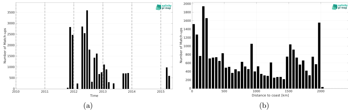
Figure 2: Number of match-ups between TSG (SAMOS) and Aquarius SSS L4 OI v5 - Monthly (IPRC) SSS as a function of time (a) and as function of the distance to coast (b) over the Amazon and Orinoco river plumes Pi-MEP region and for the full satellite product period.
