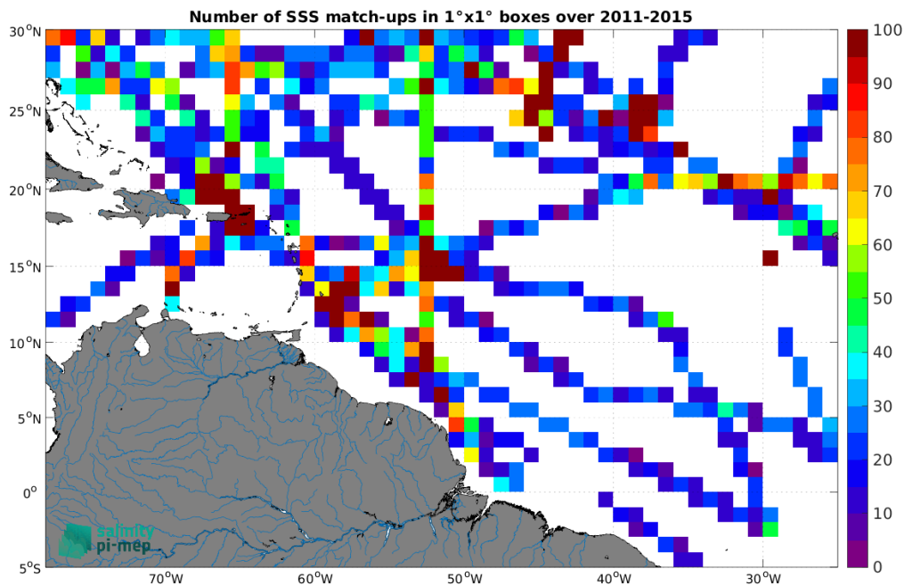
Figure 5: Number of SSS match-ups between TSG (SAMOS) SSS and the Aquarius SSS L4 OI v5 - Monthly (IPRC) SSS product for the Amazon and Orinoco river plumes Pi-MEP region over 1^\circ \times 1^\circ boxes and for the full satellite product period.
