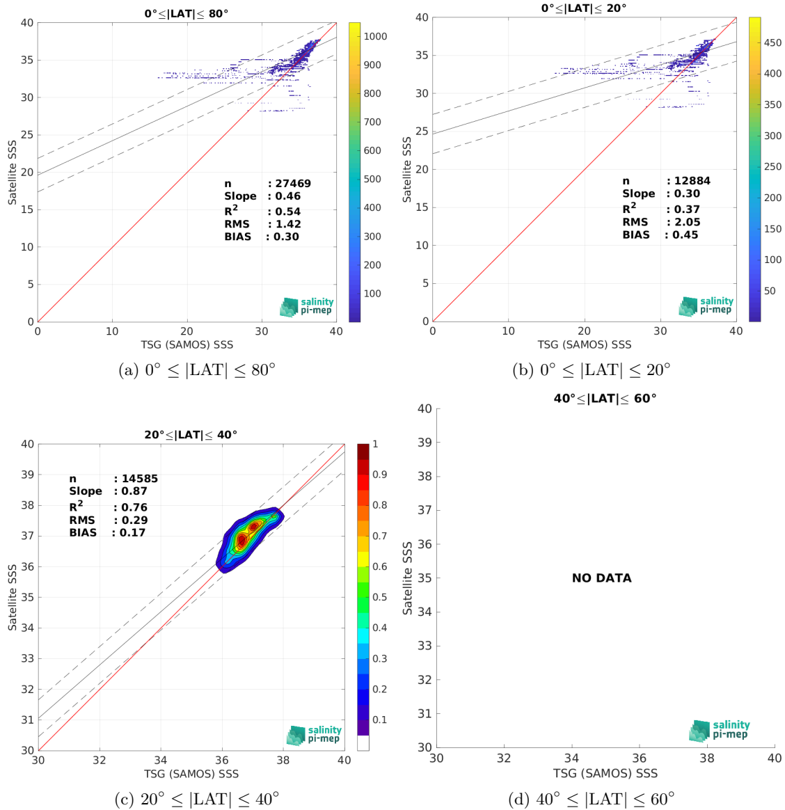
Figure 10: Contour maps of the concentration of Aquarius SSS L4 OI v5 - Monthly (IPRC) SSS (y-axis) versus TSG (SAMOS) SSS (x-axis) at match-up pairs for different latitude bands. For each plot, the red line shows x=y . The black thin and dashed lines indicate a linear fit through the data cloud and the \pm 95\% confidence levels, respectively. The number match-up pairs n , the slope and R^2 coefficient of the linear fit, the root mean square (RMS) and the mean bias between satellite and in situ data are indicated for each latitude band in each plots.
