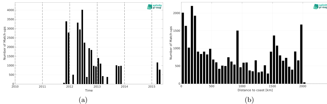
Figure 1: Number of match-ups between TSG (SAMOS) and Aquarius SSS L4 OI v5 - Monthly (IPRC) SSS as a function of time (a) and as function of the distance to coast (b) over the Amazon and Orinoco river plumes Pi-MEP region and for the full satellite product period.
