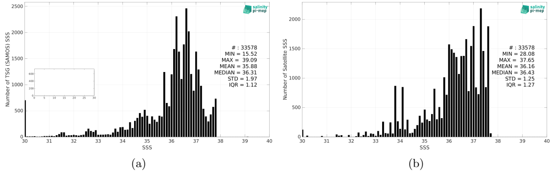
Figure 2: Histograms of SSS from TSG (SAMOS) (a) and Aquarius SSS L4 OI v5 - Monthly (IPRC) (b) considering all match-up pairs per bins of 0.1 over the Amazon and Orinoco river plumes Pi-MEP region and for the full satellite product period.
