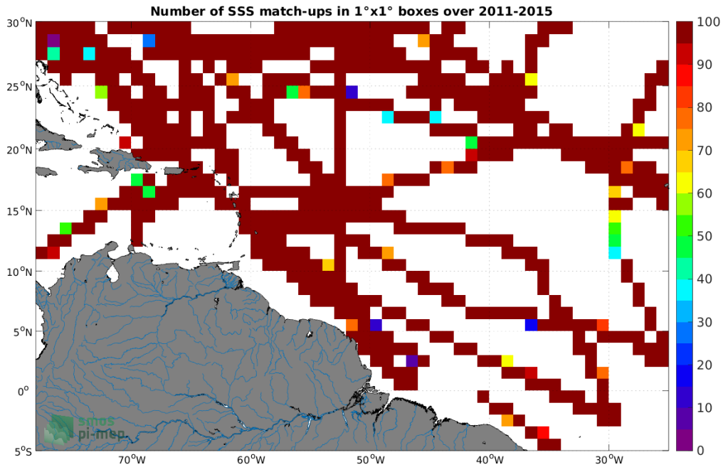
Figure 4: Number of SSS match-ups between TSG (SAMOS) SSS and the Aquarius SSS L4 OI v5 - Monthly (IPRC) SSS product for the Amazon and Orinoco river plumes Pi-MEP region over 1°×1° boxes and for the full satellite product period.
