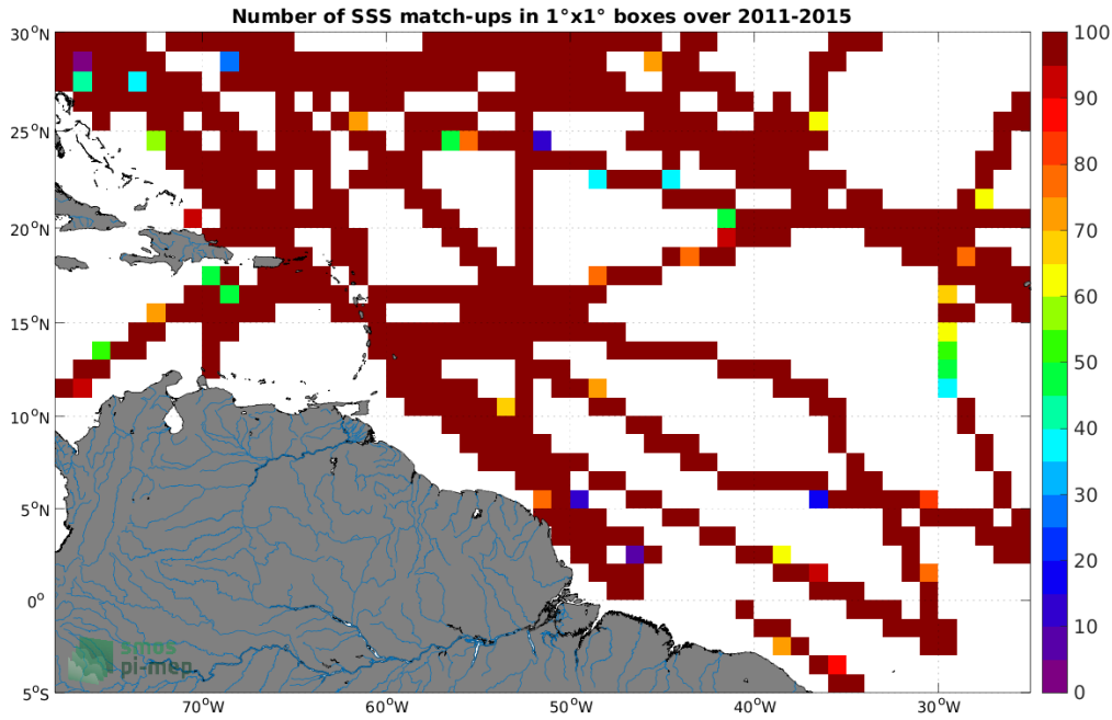
Figure 4: Number of SSS match-ups between TSG (SAMOS) SSS and the Aquarius SSS L4 OI v5 - Monthly (IPRC) SSS product for the Amazon and Orinoco river plumes Pi-MEP region over 1^{\circ} \times 1^{\circ} boxes and for the full satellite product period.
