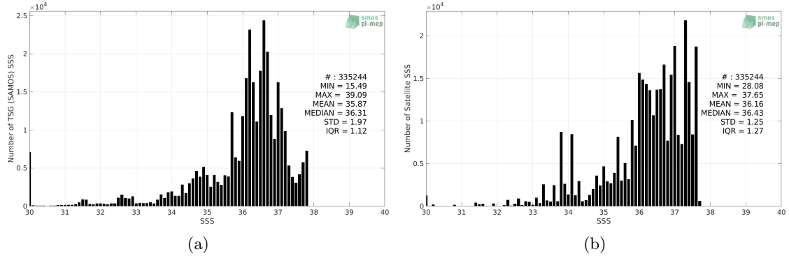
Figure 2: Histograms of SSS from TSG (SAMOS) (a) and Aquarius SSS L4 OI v5 - Monthly (IPRC) (b) considering all match-up pairs per bins of 0.1 over the Amazon and Orinoco river plumes Pi-MEP region and for the full satellite product period.
