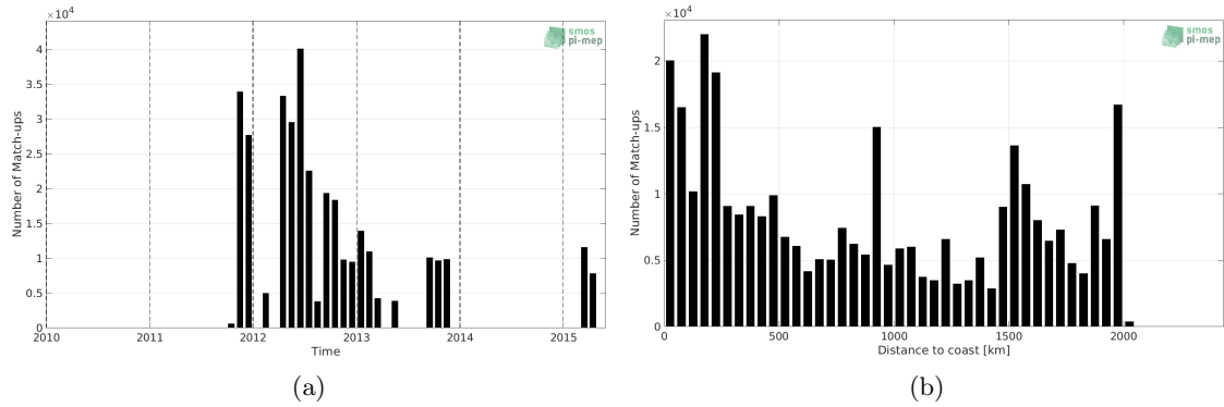
Figure 1: Number of match-ups between TSG (SAMOS) and Aquarius SSS L4 OI v5 - Monthly (IPRC) SSS as a function of time (a) and as function of the distance to coast (b) over the Amazon and Orinoco river plumes Pi-MEP region and for the full satellite product period.
