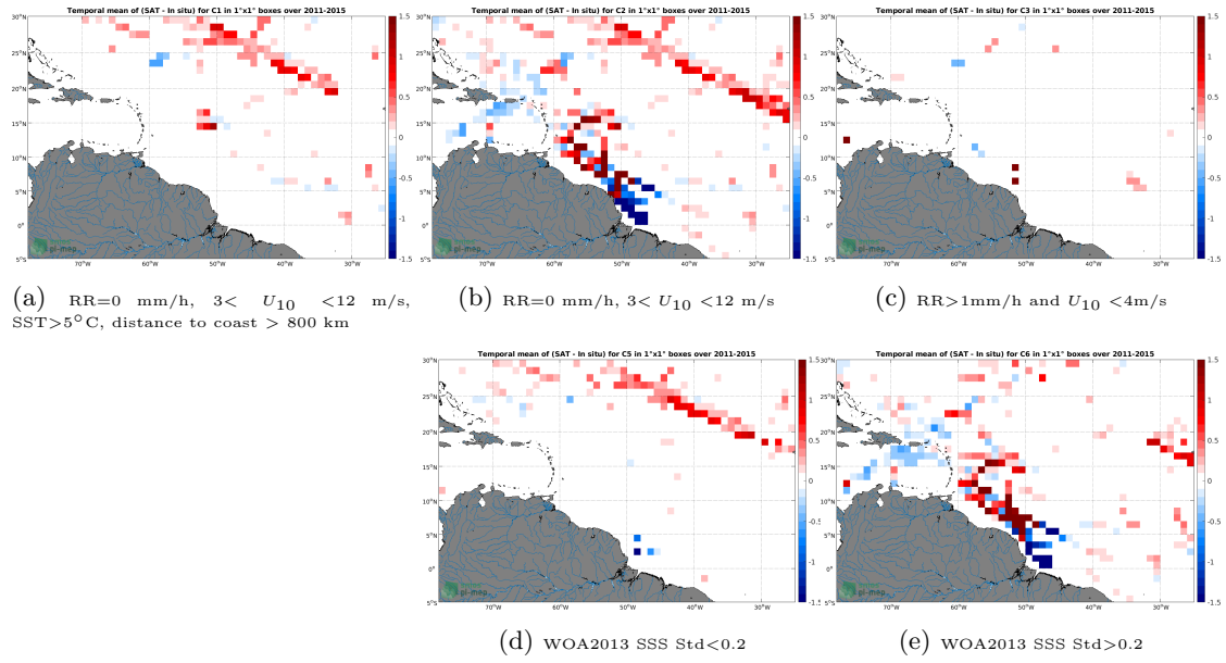
Figure 12: Temporal mean gridded over spatial boxes of size 1^\circ \times 1^\circ of \Delta SSS (Aquarius SSS L4 OI v5 - Monthly (IPRC) - TSG (SAMOS)) for 5 different subdatasets corresponding to: RR=0 mm/h, 3 < U_{10} < 12 m/s, SST > 5^\circ\text{C} , distance to coast > 800 km (a), RR=0 mm/h, 3 < U_{10} < 12 m/s (b), RR > 1 mm/h and U_{10} < 4 m/s (c), WOA2013 SSS Std < 0.2 (d), WOA2013 SSS Std > 0.2 (e).
