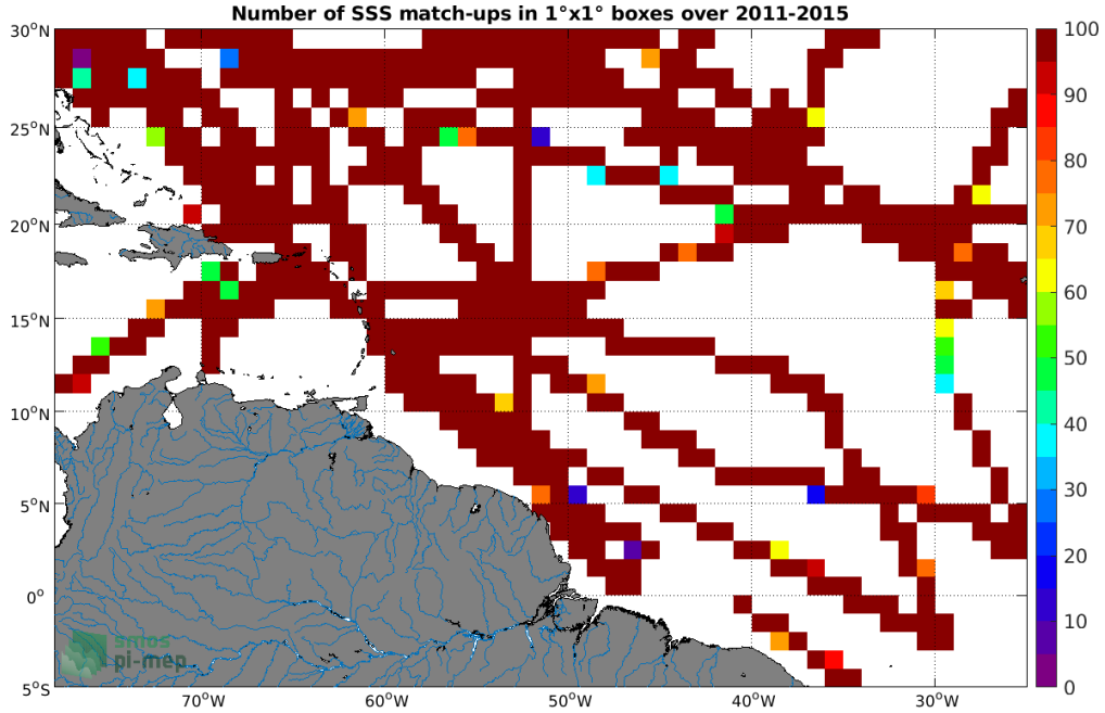
Figure 4: Number of SSS match-ups between TSG (SAMOS) SSS and the Aquarius SSS L4 OI v5 - Monthly (IPRC) SSS product for the Amazon and Orinoco river plumes Pi-MEP region over 1^\circ \times 1^\circ boxes and for the full satellite product period.
