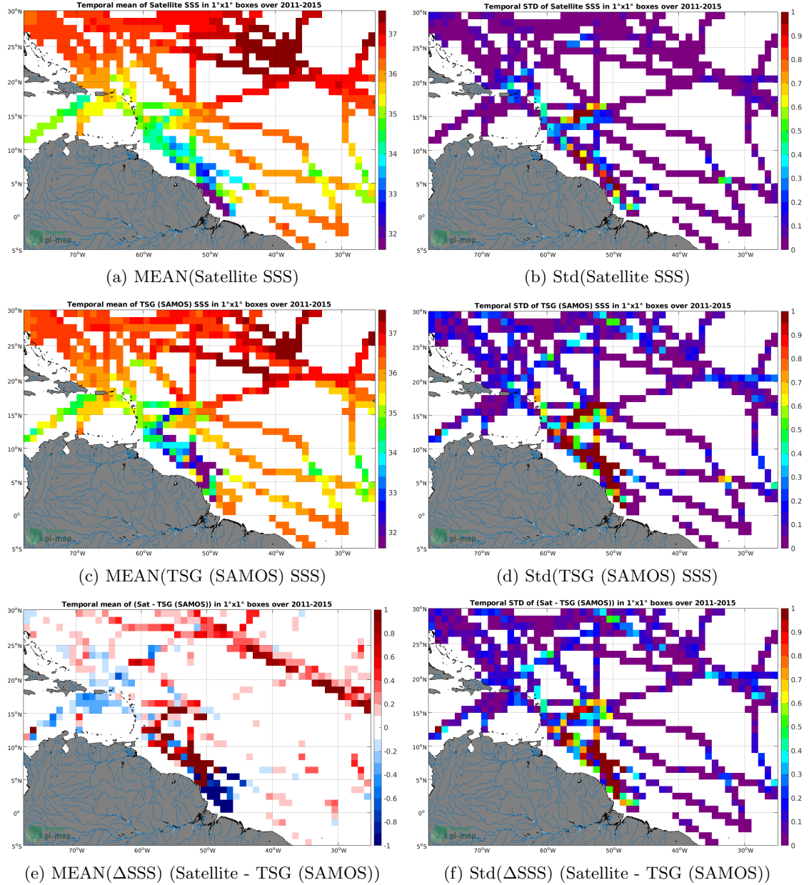
Figure 6: Temporal mean (left) and Std (right) of SSS from Aquarius SSS L4 OI v5 - Monthly (IPRC) (top), TSG (SAMOS) (middle), and of \Delta SSS (Satellite - TSG (SAMOS)). Only match-up pairs are used to generate these maps.
