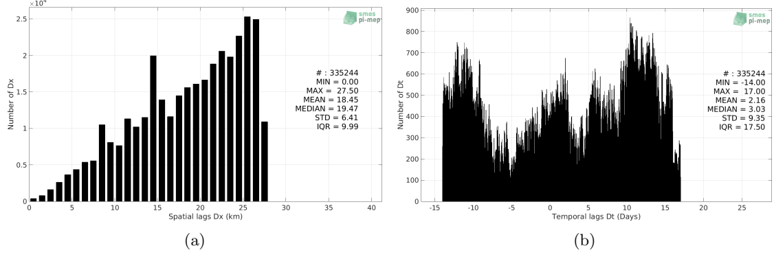
Figure 5: Histograms of the spatial (a) and temporal (b) lags between the time of the TSG (SAMOS) measurements and the date of the corresponding Aquarius SSS L4 OI v5 - Monthly (IPRC) SSS product.
