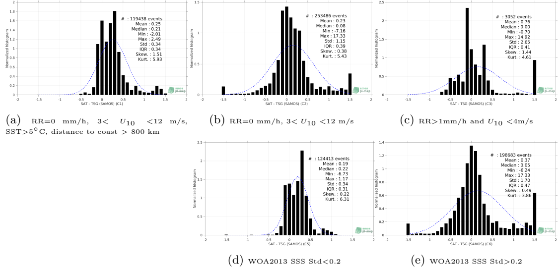
Figure 13: Normalized histogram of \Delta SSS (Aquarius SSS L4 OI v5 - Monthly (IPRC) - TSG (SAMOS)) for 5 different subdatasets corresponding to: RR=0 mm/h, 3 < U_{10} < 12 m/s, SST>5°C, distance to coast > 800 km (a), RR=0 mm/h, 3 < U_{10} < 12 m/s (b), RR>1mm/h and U_{10} < 4 m/s (c), WOA2013 SSS Std<0.2 (d), WOA2013 SSS Std>0.2 (e).
