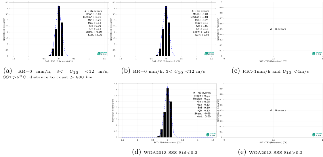
Figure 15: Normalized histogram of \Delta SSS (Aquarius SSS L4 OI v5 - Monthly (IPRC) - TSG (Polarstern)) for 5 different subdatasets corresponding to: RR=0 mm/h, 3 < U_{10} < 12 m/s, SST >5^{\circ} C, distance to coast > 800 km (a), RR=0 mm/h, 3 < U_{10} < 12 m/s (b), RR >1 mm/h and U_{10} < 4 m/s (c), WOA2013 SSS Std <0.2 (d), WOA2013 SSS Std >0.2 (e).
