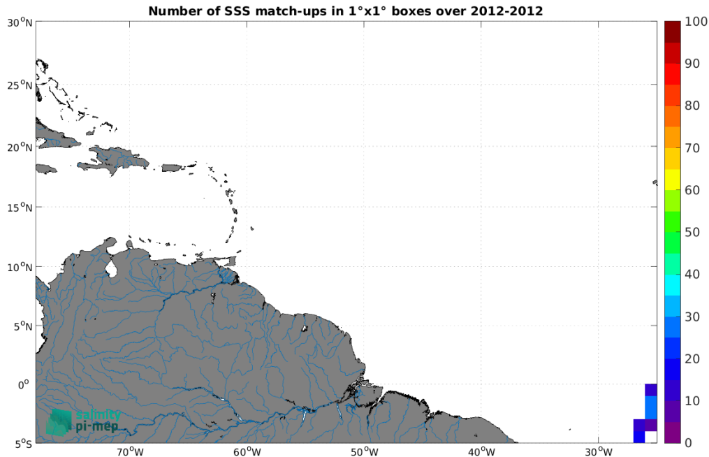
Figure 5: Number of SSS match-ups between TSG (Polarstern) SSS and the Aquarius SSS L4 OI v5 - Monthly (IPRC) SSS product for the Amazon and Orinoco river plumes Pi-MEP region over 1^\circ \times 1^\circ boxes and for the full satellite product period.
