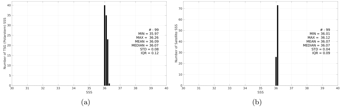
Figure 3: Histograms of SSS from TSG (Polarstern) (a) and Aquarius SSS L4 OI v5 - Monthly (IPRC) (b) considering all match-up pairs per bins of 0.1 over the Amazon and Orinoco river plumes Pi-MEP region and for the full satellite product period.
