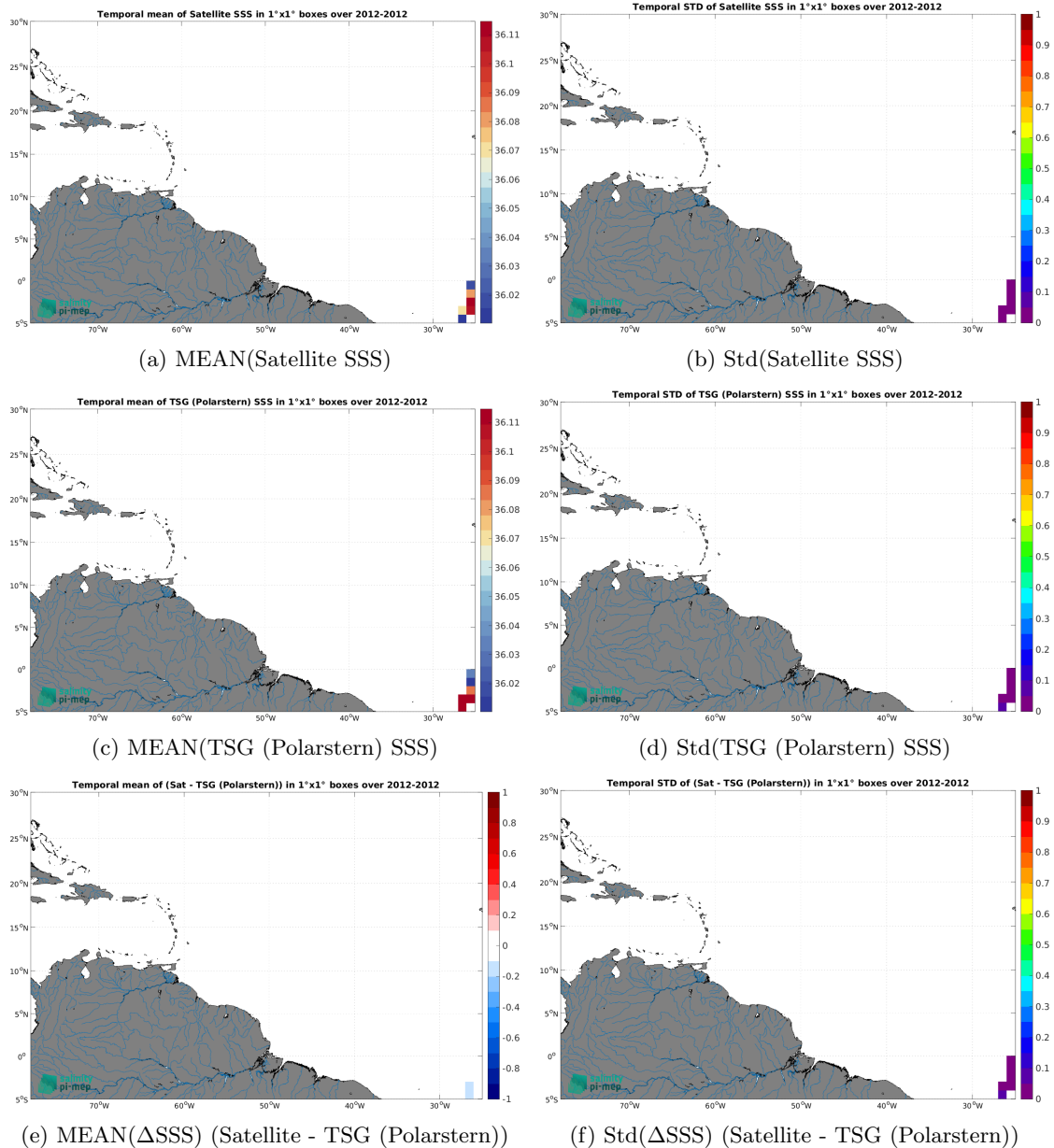
Figure 7: Temporal mean (left) and Std (right) of SSS from Aquarius SSS L4 OI v5 - Monthly (IPRC) (top), TSG (Polarstern) (middle), and of \Delta SSS (Satellite - TSG (Polarstern)). Only match-up pairs are used to generate these maps.
