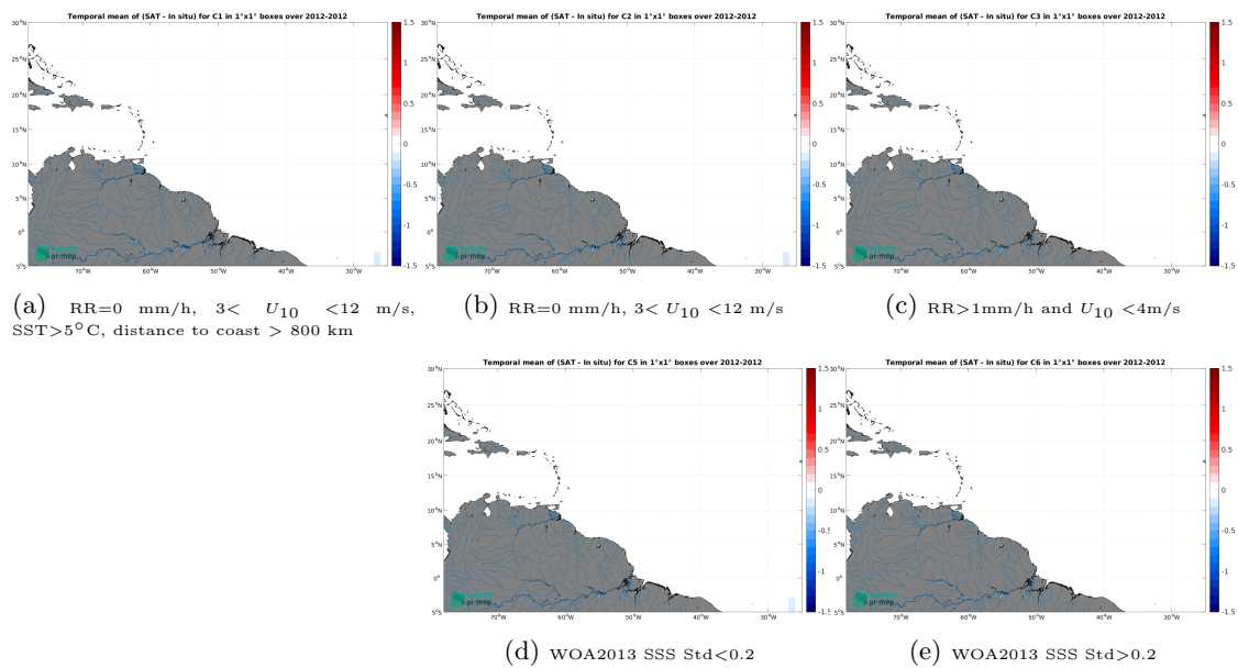
Figure 14: Temporal mean gridded over spatial boxes of size 1^\circ \times 1^\circ of \Delta SSS (Aquarius SSS L4 OI v5 - Monthly (IPRC) - TSG (Polarstern)) for 5 different subdatasets corresponding to:RR=0 mm/h, 3 < U_{10} < 12 m/s, SST >5^\circ\text{C} , distance to coast > 800 km (a), RR=0 mm/h, 3 < U_{10} < 12 m/s (b), RR >1 mm/h and U_{10} < 4 m/s (c), WOA2013 SSS Std <0.2 (d), WOA2013 SSS Std >0.2 (e).
