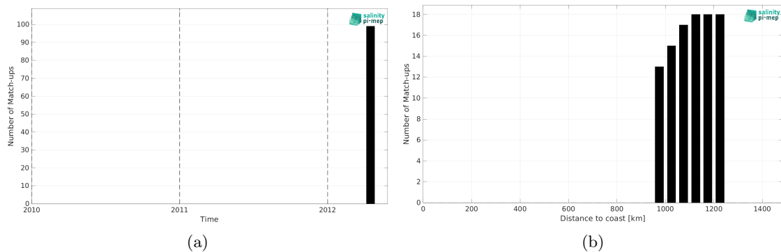
Figure 2: Number of match-ups between TSG (Polarstern) and Aquarius SSS L4 OI v5 - Monthly (IPRC) SSS as a function of time (a) and as function of the distance to coast (b) over the Amazon and Orinoco river plumes Pi-MEP region and for the full satellite product period.
