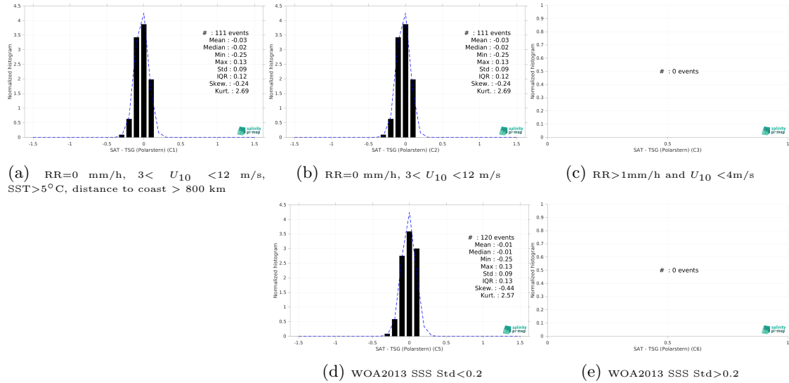
Figure 13: Normalized histogram of \Delta\text{SSS} (Aquarius SSS L4 OI v5 - Monthly (IPRC) - TSG (Polarstern)) for 5 different subdatasets corresponding to: RR=0 mm/h, 3 < U_{10} < 12 m/s, SST > 5^\circ\text{C} , distance to coast > 800 km (a), RR=0 mm/h, 3 < U_{10} < 12 m/s (b), RR > 1\text{mm/h} and U_{10} < 4\text{m/s} (c), WOA2013 SSS Std < 0.2 (d), WOA2013 SSS Std > 0.2 (e).
