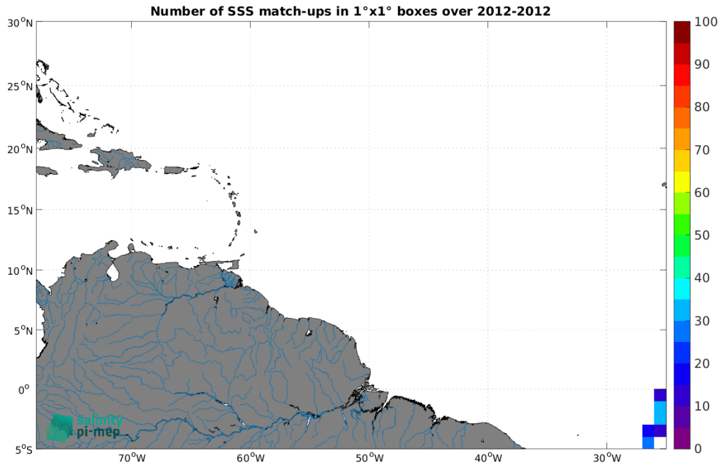
Figure 4: Number of SSS match-ups between TSG (Polarstern) SSS and the Aquarius SSS L4 OI v5 - Monthly (IPRC) SSS product for the Amazon and Orinoco river plumes Pi-MEP region over 1^{\circ} \times 1^{\circ} boxes and for the full satellite product period.
