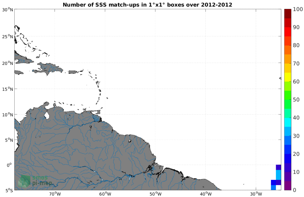
Figure 4: Number of SSS match-ups between TSG (Polarstern) SSS and the Aquarius SSS L4 OI v5 - Monthly (IPRC) SSS product for the Amazon and Orinoco river plumes Pi-MEP region over 1°×1° boxes and for the full satellite product period.
