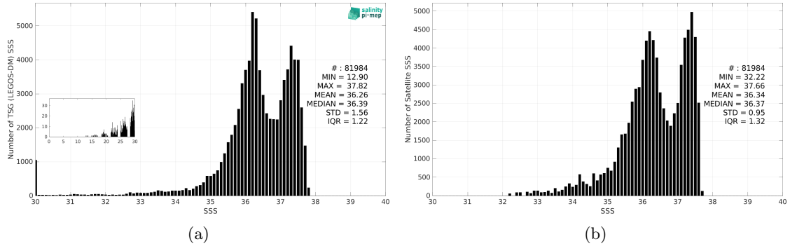
Figure 3: Histograms of SSS from TSG (LEGOS-DM) (a) and Aquarius SSS L4 OI v5 - Monthly (IPRC) (b) considering all match-up pairs per bins of 0.1 over the Amazon and Orinoco river plumes Pi-MEP region and for the full satellite product period.
