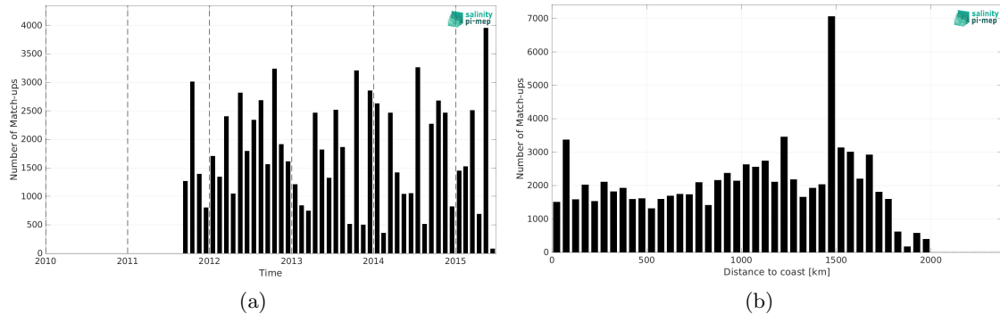
Figure 2: Number of match-ups between TSG (LEGOS-DM) and Aquarius SSS L4 OI v5 - Monthly (IPRC) SSS as a function of time (a) and as function of the distance to coast (b) over the Amazon and Orinoco river plumes Pi-MEP region and for the full satellite product period.
