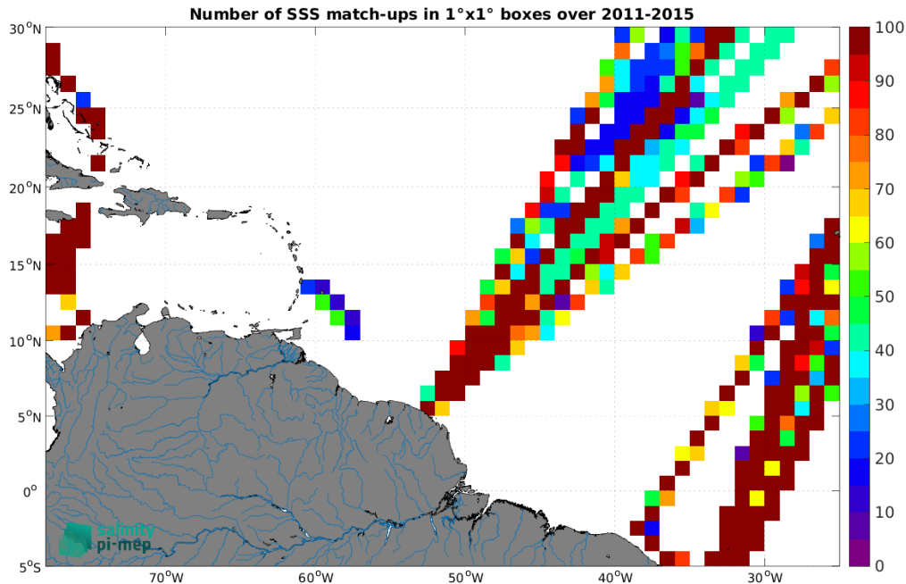
Figure 5: Number of SSS match-ups between TSG (LEGOS-DM) SSS and the Aquarius SSS L4 OI v5 - Monthly (IPRC) SSS product for the Amazon and Orinoco river plumes Pi-MEP region over 1^\circ \times 1^\circ boxes and for the full satellite product period.
