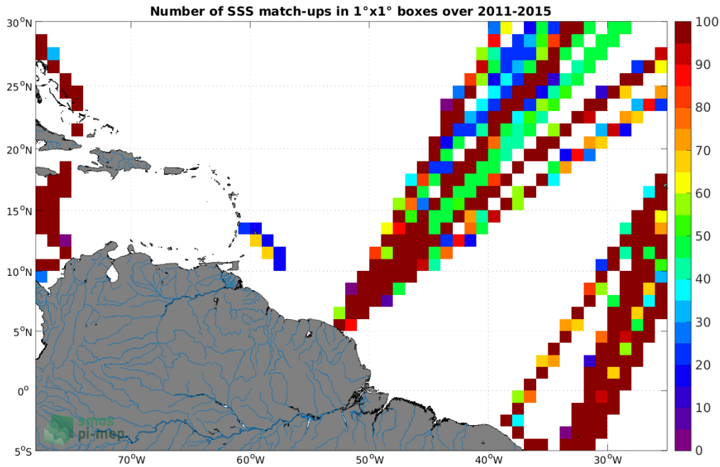
Figure 4: Number of SSS match-ups between TSG (LEGOS-DM) SSS and the Aquarius SSS L4 OI v5 - Monthly (IPRC) SSS product for the Amazon and Orinoco river plumes Pi-MEP region over 1°×1° boxes and for the full satellite product period.
