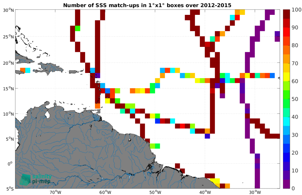
Figure 5: Number of SSS match-ups between TSG (GOSUD-Sailing-ship) SSS and the Aquarius SSS L4 OI v5 - Monthly (IPRC) SSS product for the Amazon and Orinoco river plumes Pi-MEP region over 1^\circ \times 1^\circ boxes and for the full satellite product period.
