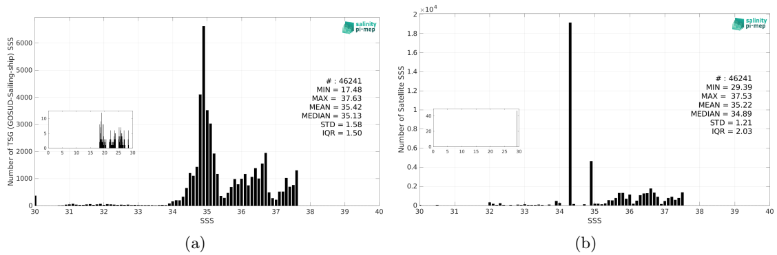
Figure 3: Histograms of SSS from TSG (GOSUD-Sailing-ship) (a) and Aquarius SSS L4 OI v5 - Monthly (IPRC) (b) considering all match-up pairs per bins of 0.1 over the Amazon and Orinoco river plumes Pi-MEP region and for the full satellite product period.
