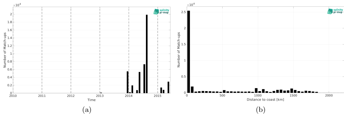
Figure 2: Number of match-ups between TSG (GOSUD-Sailing-ship) and Aquarius SSS L4 OI v5 - Monthly (IPRC) SSS as a function of time (a) and as function of the distance to coast (b) over the Amazon and Orinoco river plumes Pi-MEP region and for the full satellite product period.
