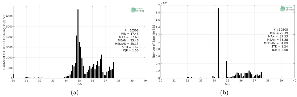
Figure 2: Histograms of SSS from TSG (GOSUD-Sailing-ship) (a) and Aquarius SSS L4 OI v5 - Monthly (IPRC) (b) considering all match-up pairs per bins of 0.1 over the Amazon and Orinoco river plumes Pi-MEP region and for the full satellite product period.
