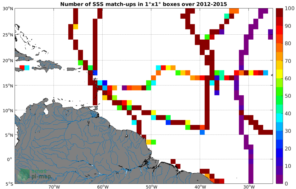
Figure 4: Number of SSS match-ups between TSG (GOSUD-Sailing-ship) SSS and the Aquarius SSS L4 OI v5 - Monthly (IPRC) SSS product for the Amazon and Orinoco river plumes Pi-MEP region over 1^\circ \times 1^\circ boxes and for the full satellite product period.
