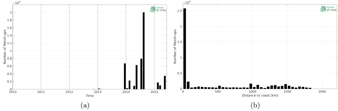
Figure 1: Number of match-ups between TSG (GOSUD-Sailing-ship) and Aquarius SSS L4 OI v5 - Monthly (IPRC) SSS as a function of time (a) and as function of the distance to coast (b) over the Amazon and Orinoco river plumes Pi-MEP region and for the full satellite product period.
