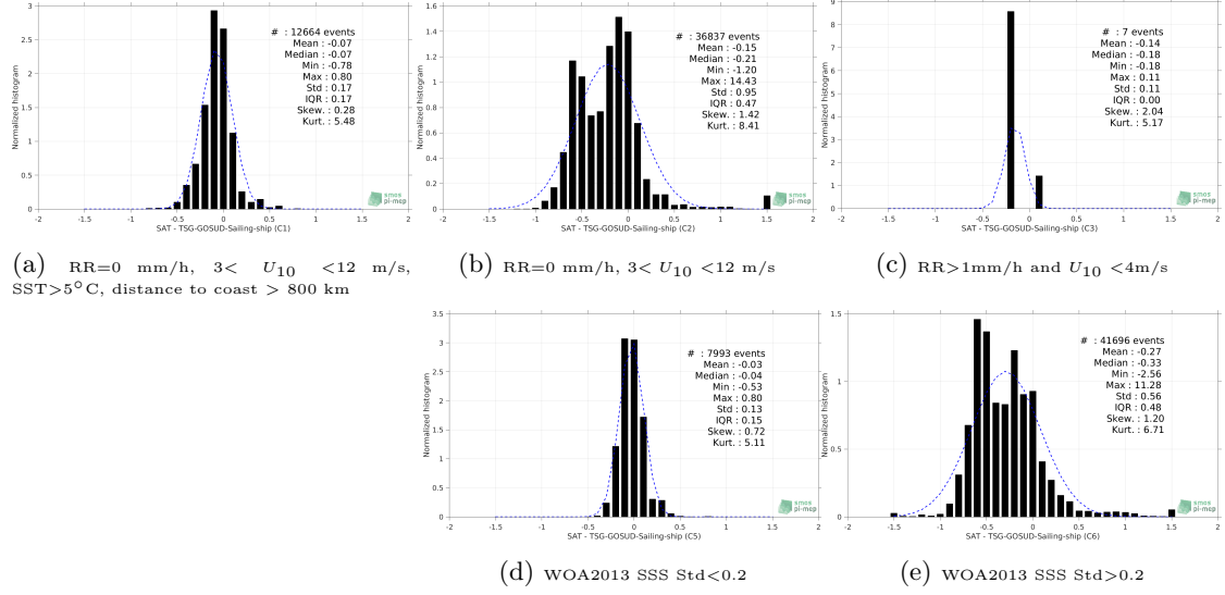
Figure 13: Normalized histogram of \Delta\text{SSS} (Aquarius-L4-IPRC-V5-MONTHLY - TSG-GOSUD-Sailing-ship) for 5 different subdatasets corresponding to: RR=0 mm/h, 3 < U_{10} < 12 m/s, SST > 5^\circ\text{C} , distance to coast > 800 km (a), RR=0 mm/h, 3 < U_{10} < 12 m/s (b), RR > 1\text{mm/h} and U_{10} < 4\text{m/s} (c), WOA2013 SSS Std < 0.2 (d), WOA2013 SSS Std > 0.2 (e).
